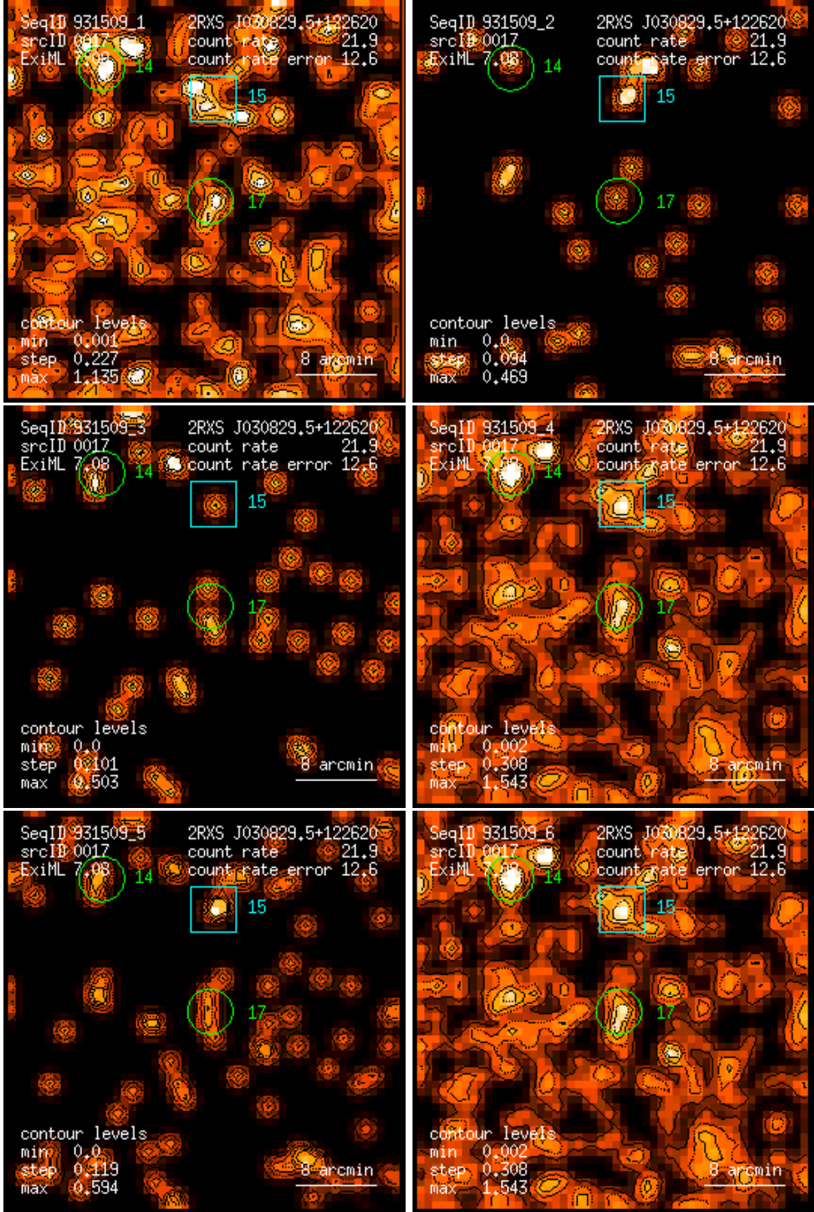
Figure 17: RASS 931509: detection 0017: band rate images, Gaussian filter: (1) PSPC channels 11 – 41, (2) 52 – 90, (3) 91 – 201, (4) 11 – 235, (5) 52 – 201, (6) 11 – 201. Broad band rates in counts/ks. Band rate contour levels in counts/ks/arcmin 2 .
