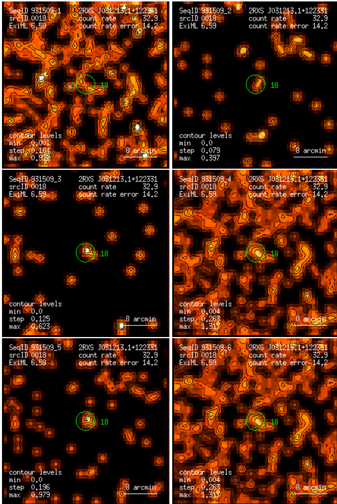
Figure 18: RASS 931509: detection 0018: band rate images, Gaussian filter: (1) PSPC channels 11 – 41, (2) 52 – 90, (3) 91 – 201, (4) 11 – 235, (5) 52 – 201, (6) 11 – 201. Broad band rates in counts/ks. Band rate contour levels in counts/ks/arcmin 2 .
