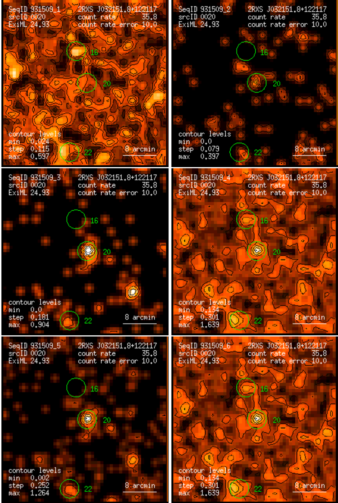
Figure 20: RASS 931509: detection 0020: band rate images, Gaussian filter: (1) PSPC channels 11 – 41, (2) 52 – 90, (3) 91 – 201, (4) 11 – 235, (5) 52 – 201, (6) 11 – 201. Broad band rates in counts/ks. Band rate contour levels in counts/ks/arcmin 2 .
