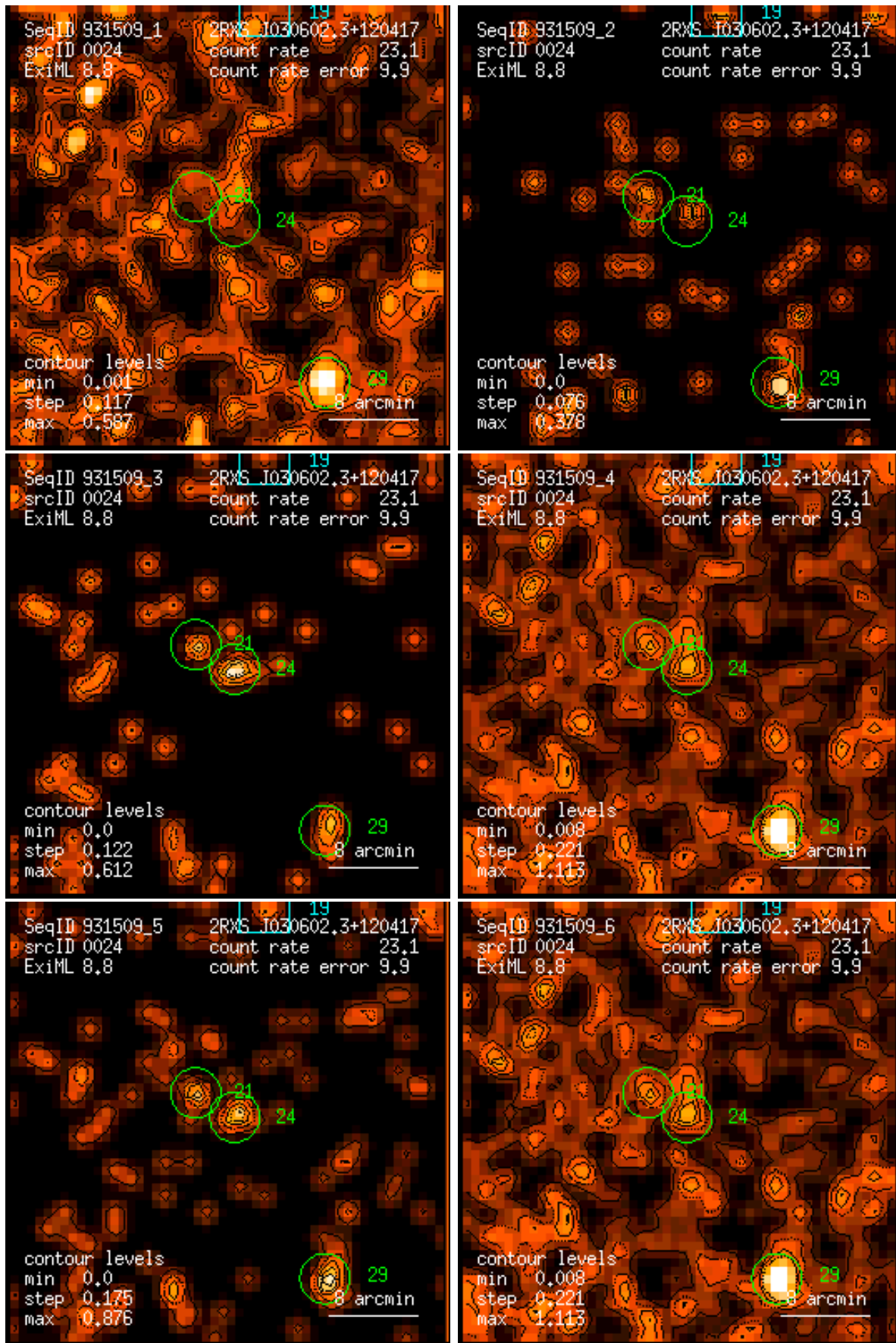
Figure 24: RASS 931509: detection 0024: band rate images, Gaussian filter: (1) PSPC channels 11 – 41, (2) 52 – 90, (3) 91 – 201, (4) 11 – 235, (5) 52 – 201, (6) 11 – 201. Broad band rates in counts/ks. Band rate contour levels in counts/ks/arcmin 2 .
