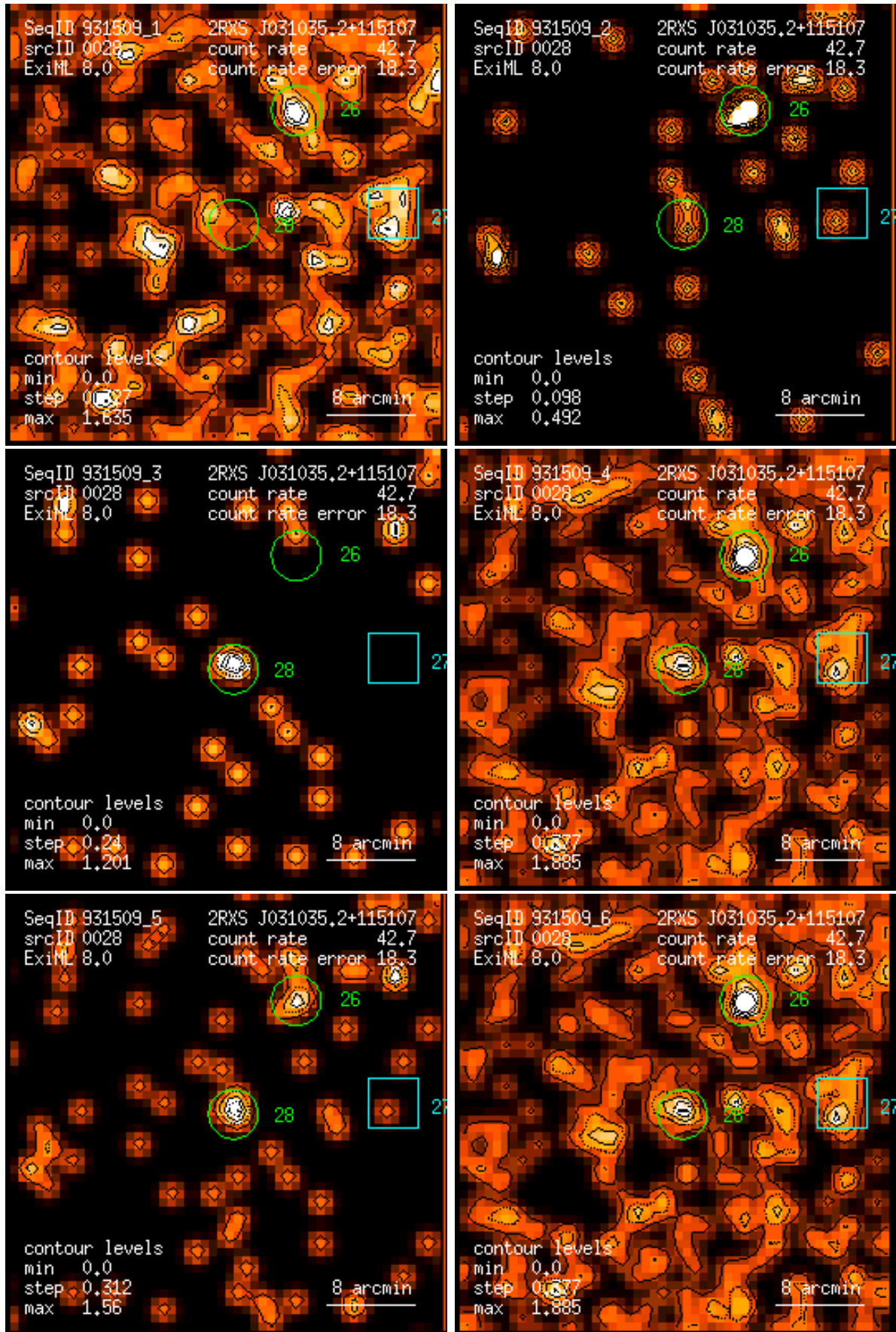
Figure 28: RASS 931509: detection 0028: band rate images, Gaussian filter: (1) PSPC channels 11 – 41, (2) 52 – 90, (3) 91 – 201, (4) 11 – 235, (5) 52 – 201, (6) 11 – 201. Broad band rates in counts/ks. Band rate contour levels in counts/ks/arcmin 2 .
