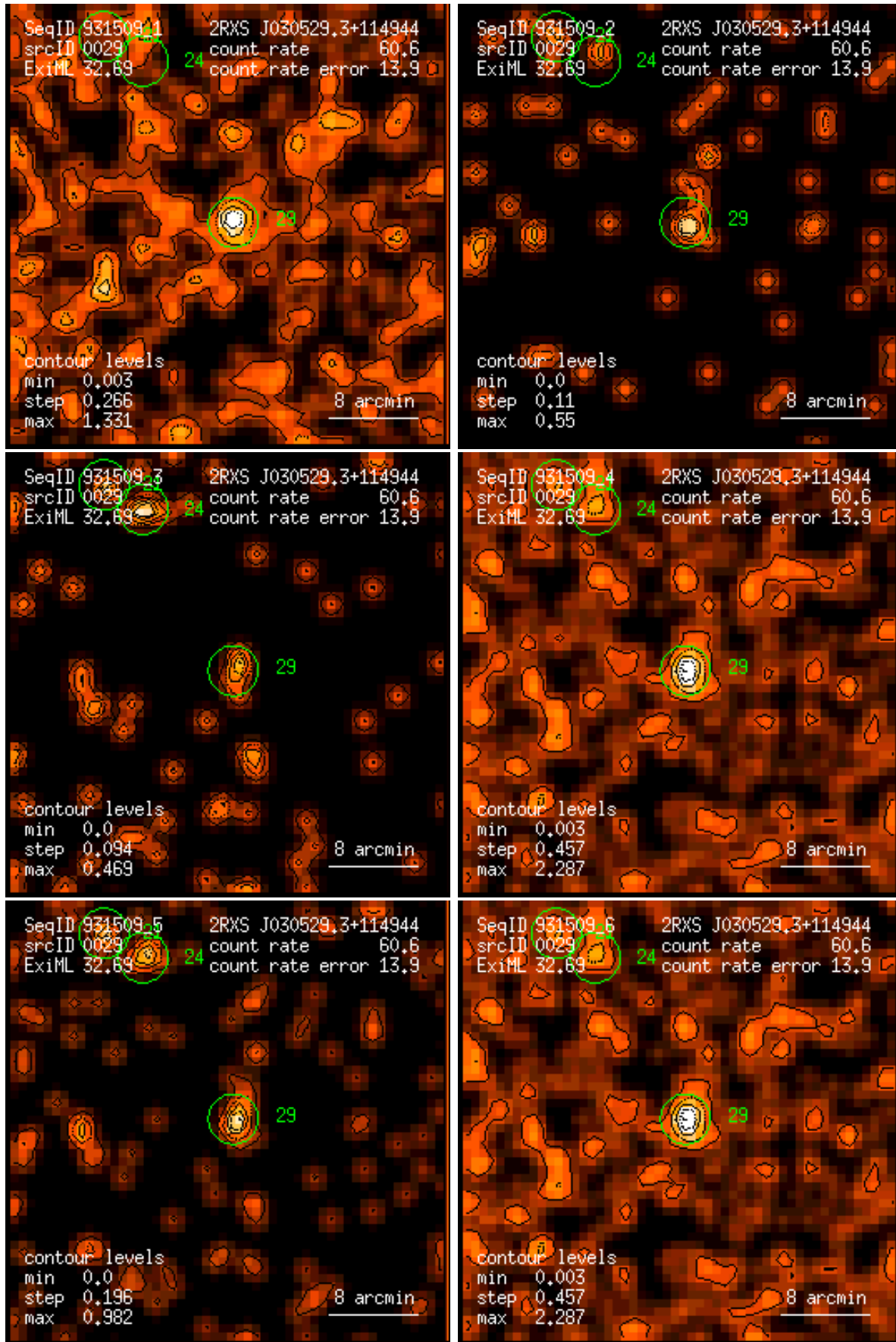
Figure 29: RASS 931509: detection 0029: band rate images, Gaussian filter: (1) PSPC channels 11 – 41, (2) 52 – 90, (3) 91 – 201, (4) 11 – 235, (5) 52 – 201, (6) 11 – 201. Broad band rates in counts/ks. Band rate contour levels in counts/ks/arcmin 2 .
