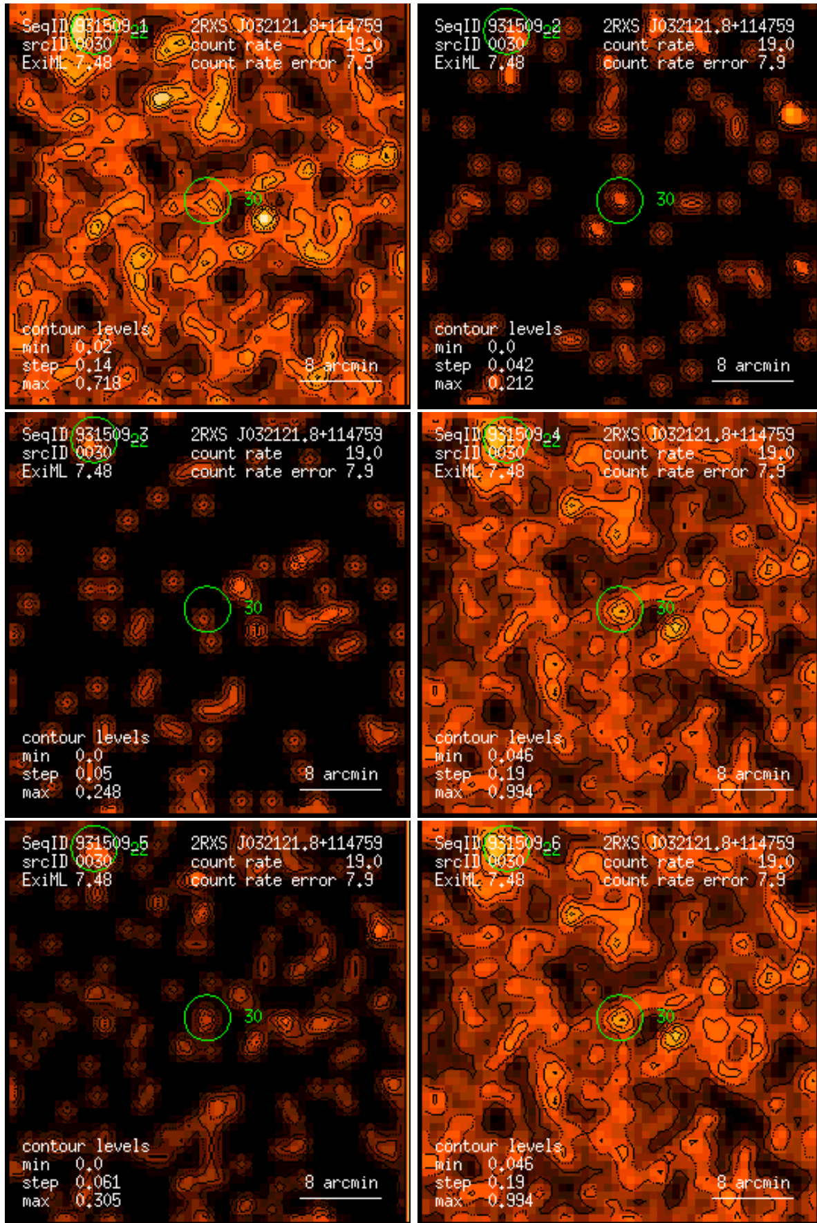
Figure 30: RASS 931509: detection 0030: band rate images, Gaussian filter: (1) PSPC channels 11 – 41, (2) 52 – 90, (3) 91 – 201, (4) 11 – 235, (5) 52 – 201, (6) 11 – 201. Broad band rates in counts/ks. Band rate contour levels in counts/ks/arcmin 2 .
