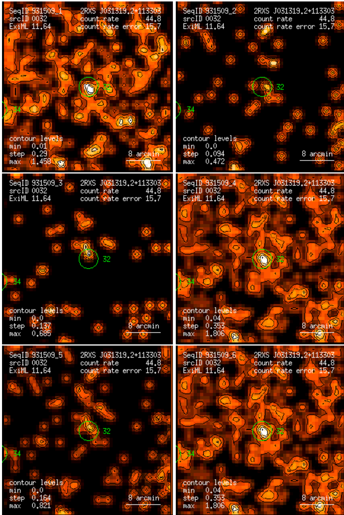
Figure 32: RASS 931509: detection 0032: band rate images, Gaussian filter: (1) PSPC channels 11 – 41, (2) 52 – 90, (3) 91 – 201, (4) 11 – 235, (5) 52 – 201, (6) 11 – 201. Broad band rates in counts/ks. Band rate contour levels in counts/ks/arcmin 2 .
