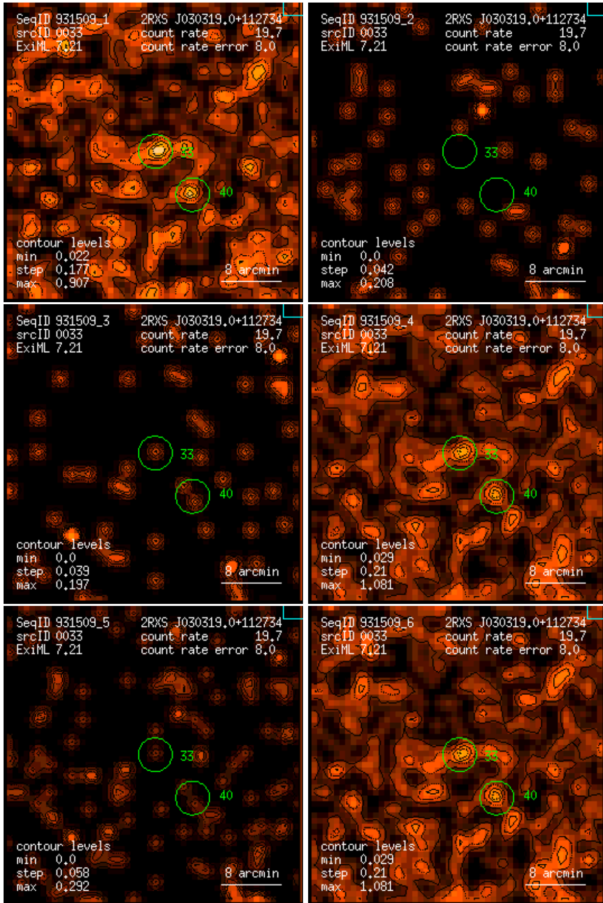
Figure 33: RASS 931509: detection 0033: band rate images, Gaussian filter: (1) PSPC channels 11 – 41, (2) 52 – 90, (3) 91 – 201, (4) 11 – 235, (5) 52 – 201, (6) 11 – 201. Broad band rates in counts/ks. Band rate contour levels in counts/ks/arcmin 2 .
