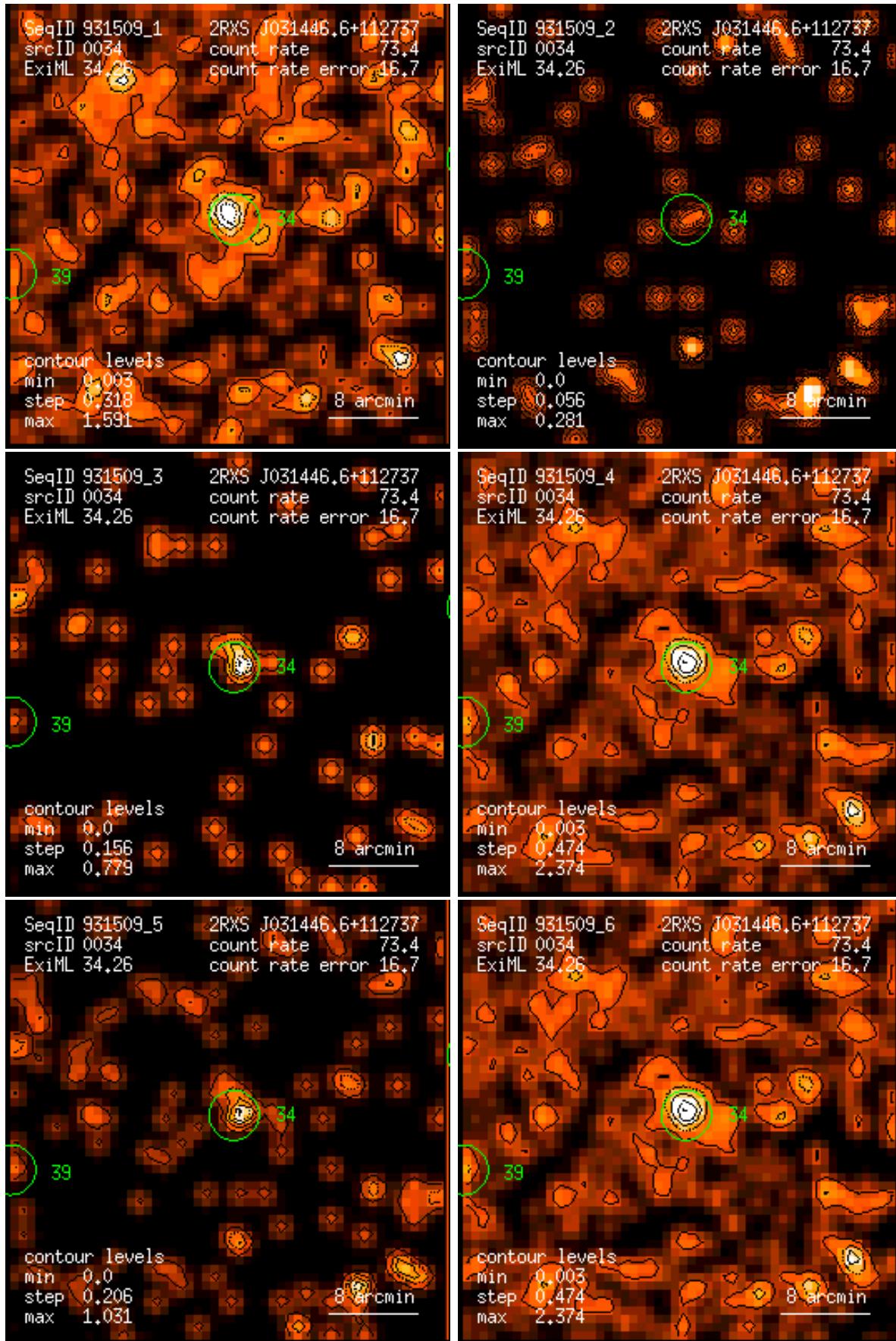
Figure 34: RASS 931509: detection 0034: band rate images, Gaussian filter: (1) PSPC channels 11 – 41, (2) 52 – 90, (3) 91 – 201, (4) 11 – 235, (5) 52 – 201, (6) 11 – 201. Broad band rates in counts/ks. Band rate contour levels in counts/ks/arcmin 2 .
