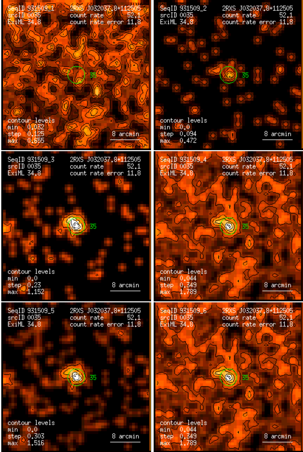
Figure 35: RASS 931509: detection 0035: band rate images, Gaussian filter: (1) PSPC channels 11 – 41, (2) 52 – 90, (3) 91 – 201, (4) 11 – 235, (5) 52 – 201, (6) 11 – 201. Broad band rates in counts/ks. Band rate contour levels in counts/ks/arcmin 2 .
