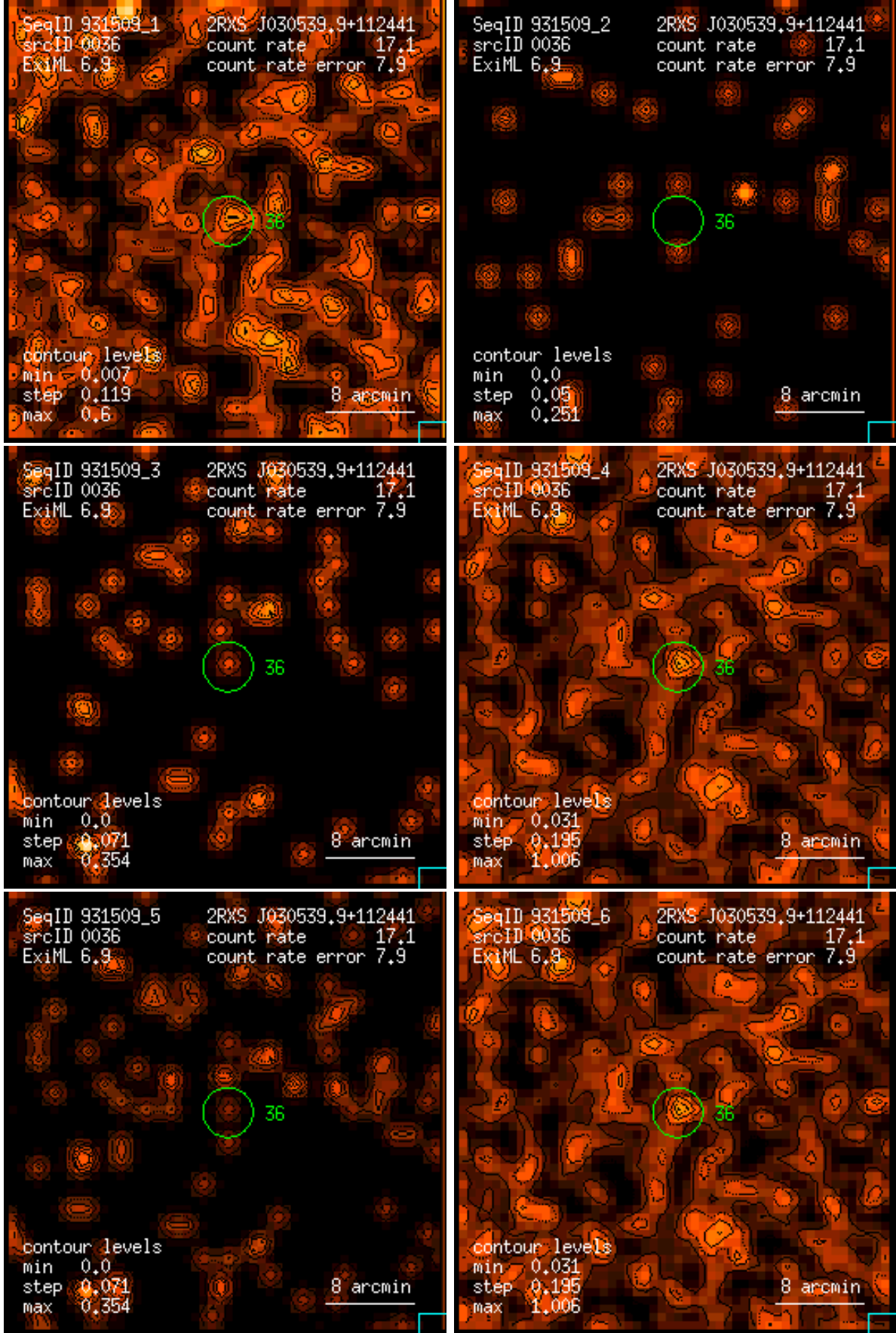
Figure 36: RASS 931509: detection 0036: band rate images, Gaussian filter: (1) PSPC channels 11 – 41, (2) 52 – 90, (3) 91 – 201, (4) 11 – 235, (5) 52 – 201, (6) 11 – 201. Broad band rates in counts/ks. Band rate contour levels in counts/ks/arcmin 2 .
