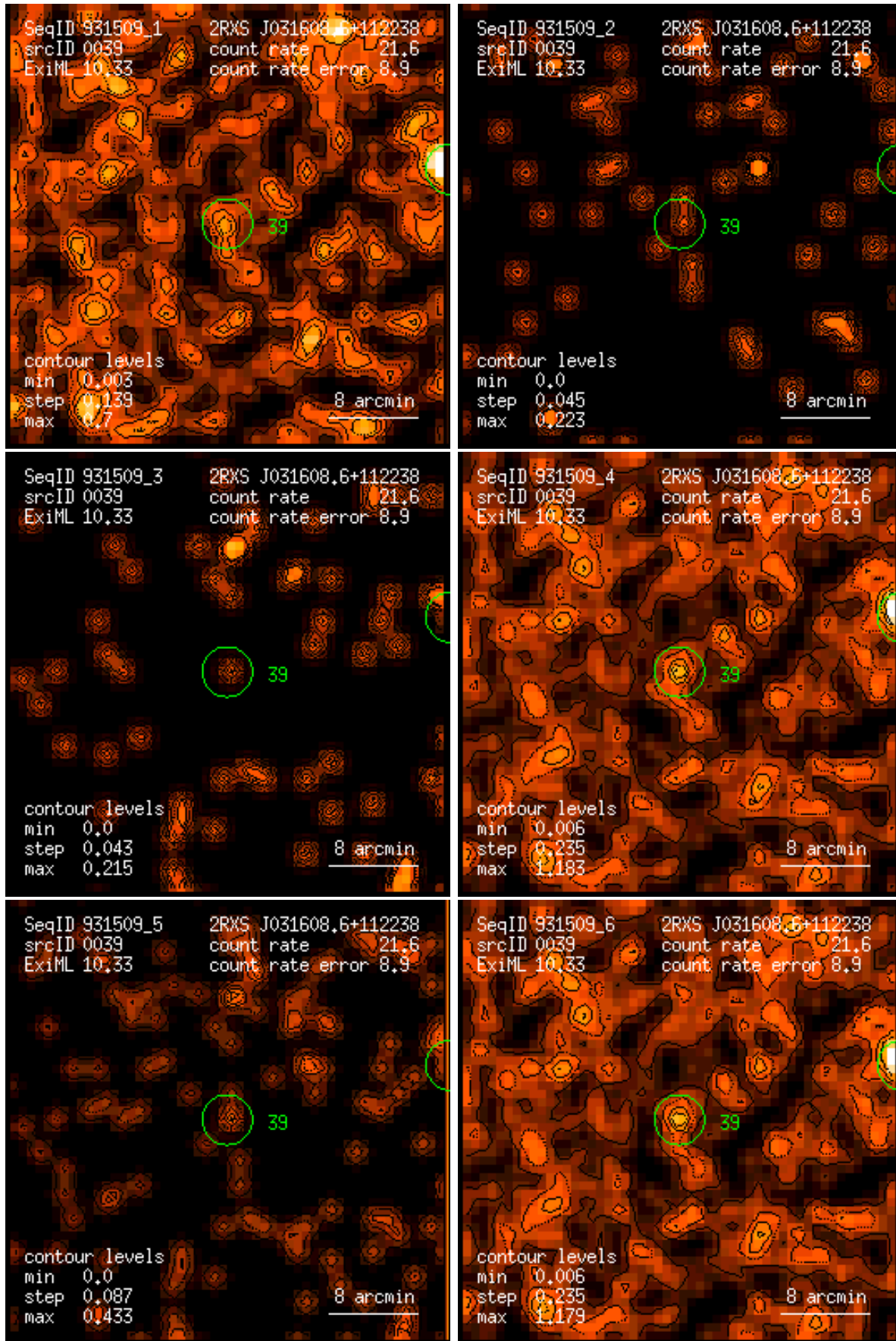
Figure 39: RASS 931509: detection 0039: band rate images, Gaussian filter: (1) PSPC channels 11 – 41, (2) 52 – 90, (3) 91 – 201, (4) 11 – 235, (5) 52 – 201, (6) 11 – 201. Broad band rates in counts/ks. Band rate contour levels in counts/ks/arcmin 2 .
