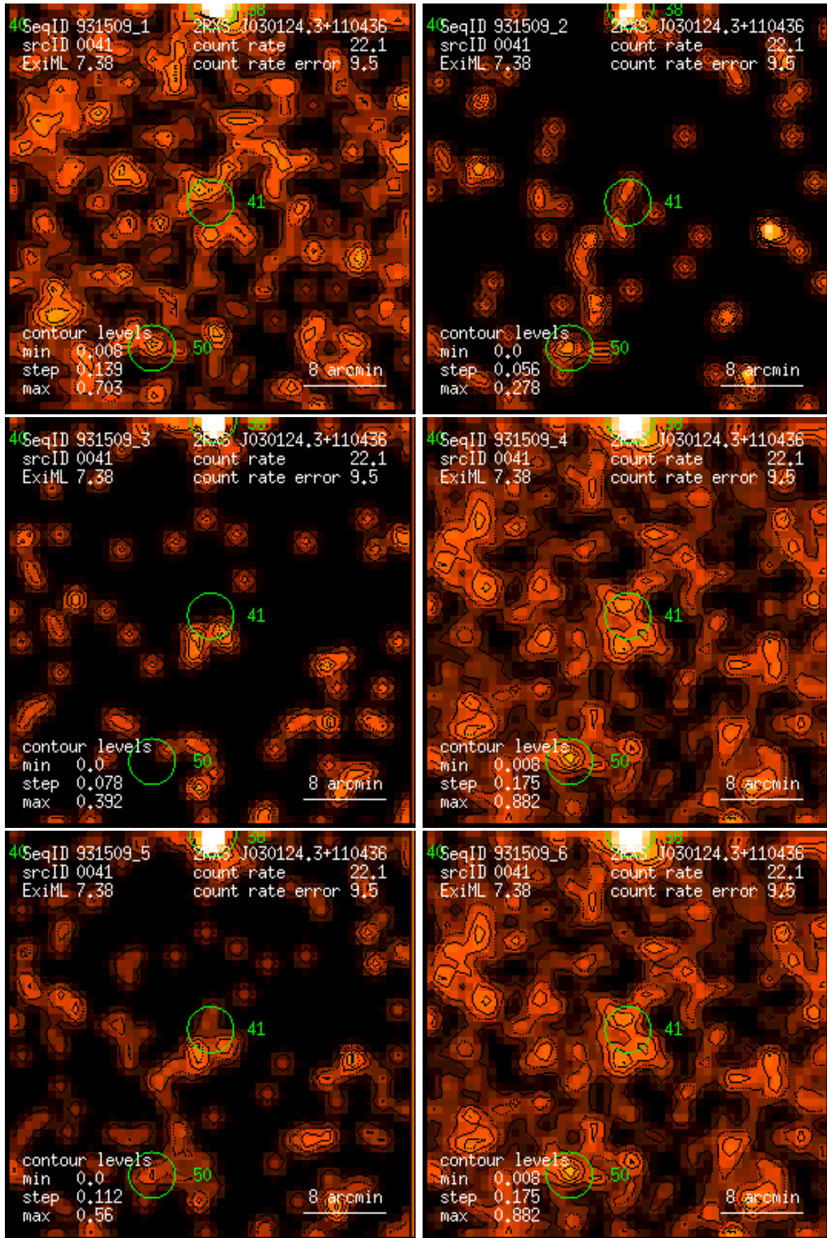
Figure 41: RASS 931509: detection 0041: band rate images, Gaussian filter: (1) PSPC channels 11 – 41, (2) 52 – 90, (3) 91 – 201, (4) 11 – 235, (5) 52 – 201, (6) 11 – 201. Broad band rates in counts/ks. Band rate contour levels in counts/ks/arcmin 2 .
