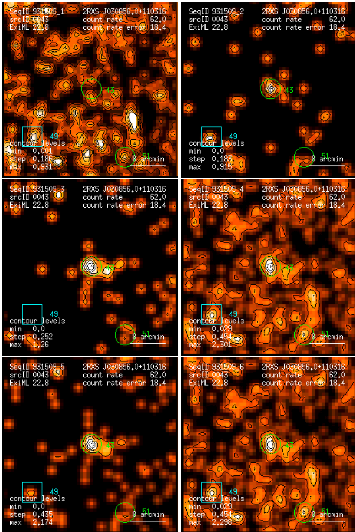
Figure 43: RASS 931509: detection 0043: band rate images, Gaussian filter: (1) PSPC channels 11 – 41, (2) 52 – 90, (3) 91 – 201, (4) 11 – 235, (5) 52 – 201, (6) 11 – 201. Broad band rates in counts/ks. Band rate contour levels in counts/ks/arcmin 2 .
