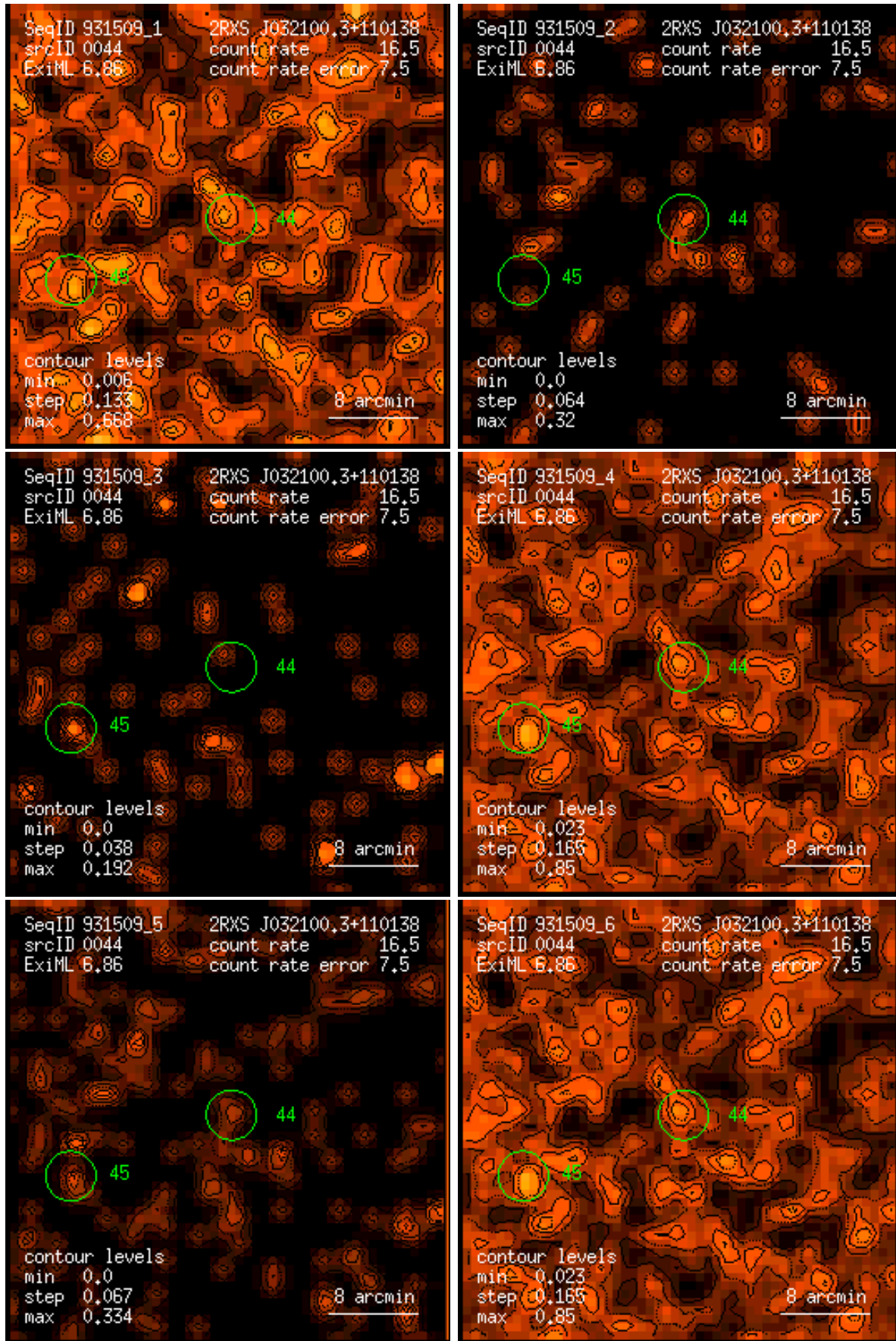
Figure 44: RASS 931509: detection 0044: band rate images, Gaussian filter: (1) PSPC channels 11 – 41, (2) 52 – 90, (3) 91 – 201, (4) 11 – 235, (5) 52 – 201, (6) 11 – 201. Broad band rates in counts/ks. Band rate contour levels in counts/ks/arcmin 2 .
