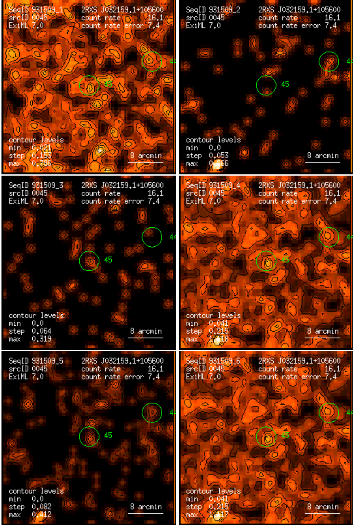
Figure 45: RASS 931509: detection 0045: band rate images, Gaussian filter: (1) PSPC channels 11 – 41, (2) 52 – 90, (3) 91 – 201, (4) 11 – 235, (5) 52 – 201, (6) 11 – 201. Broad band rates in counts/ks. Band rate contour levels in counts/ks/arcmin 2 .
