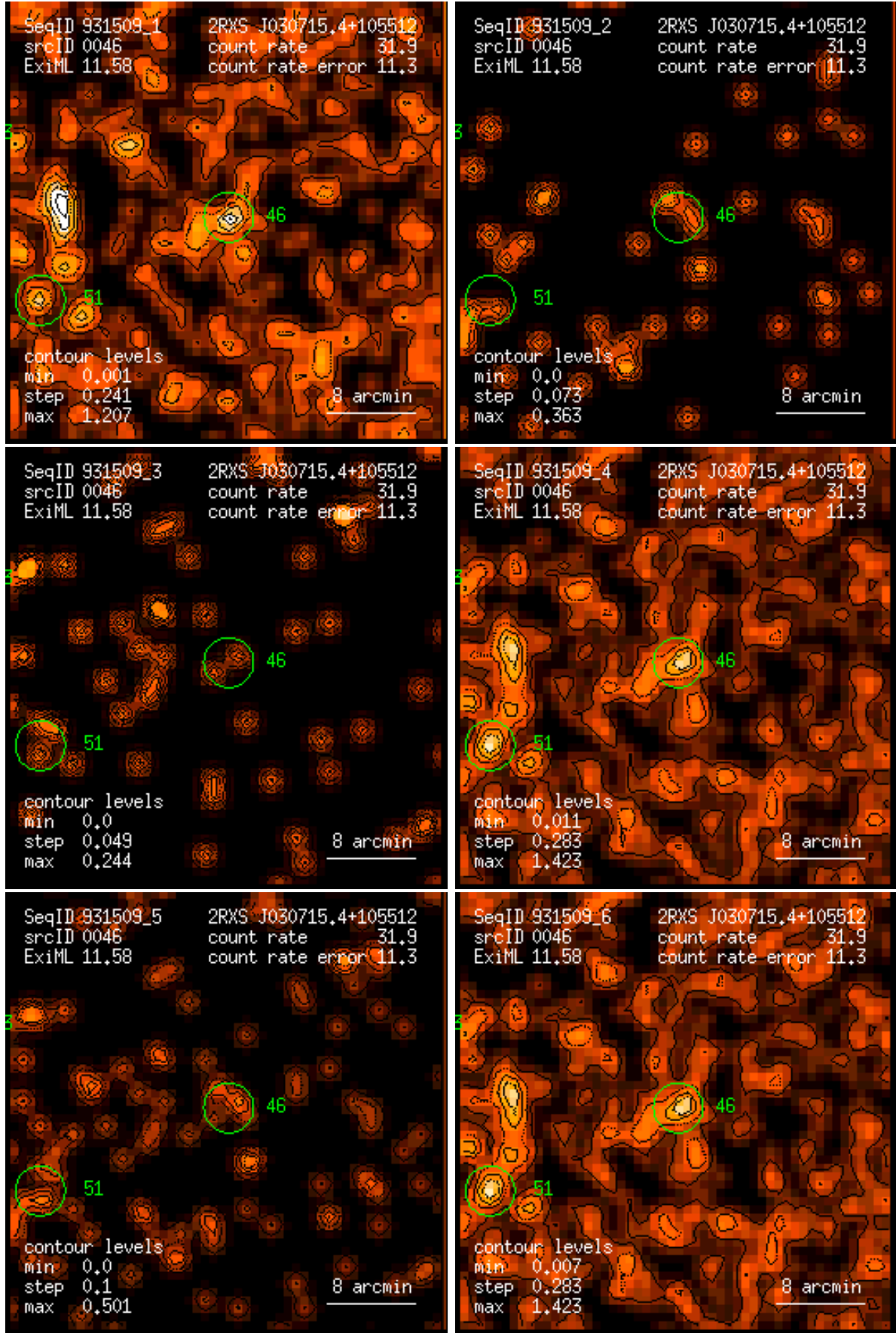
Figure 46: RASS 931509: detection 0046: band rate images, Gaussian filter: (1) PSPP channels 11 – 41, (2) 52 – 90, (3) 91 – 201, (4) 11 – 235, (5) 52 – 201, (6) 11 – 201. Broad band rates in counts/ks. Band rate contour levels in counts/ks/arcmin 2 .
