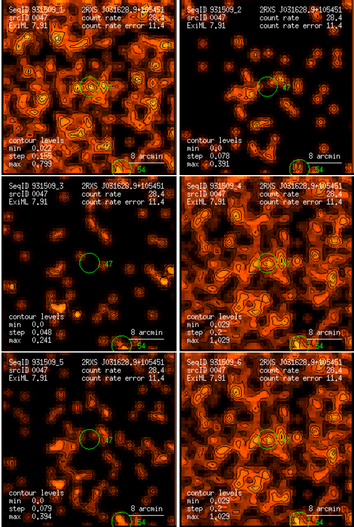
Figure 47: RASS 931509: detection 0047: band rate images, Gaussian filter: (1) PSPC channels 11 – 41, (2) 52 – 90, (3) 91 – 201, (4) 11 – 235, (5) 52 – 201, (6) 11 – 201. Broad band rates in counts/ks. Band rate contour levels in counts/ks/arcmin 2 .
