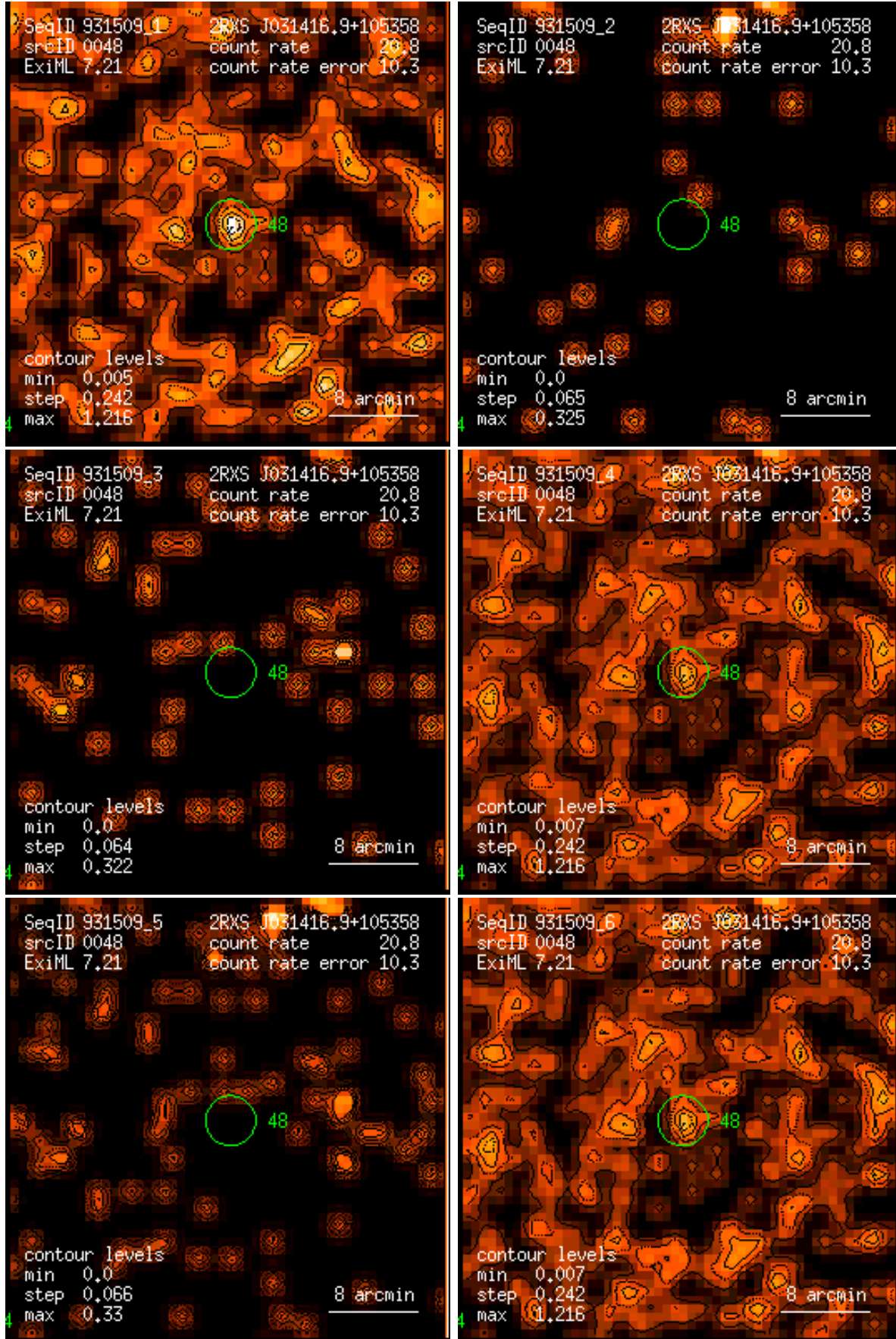
Figure 48: RASS 931509: detection 0048: band rate images, Gaussian filter: (1) PSPC channels 11 – 41, (2) 52 – 90, (3) 91 – 201, (4) 11 – 235, (5) 52 – 201, (6) 11 – 201. Broad band rates in counts/ks. Band rate contour levels in counts/ks/arcmin 2 .
