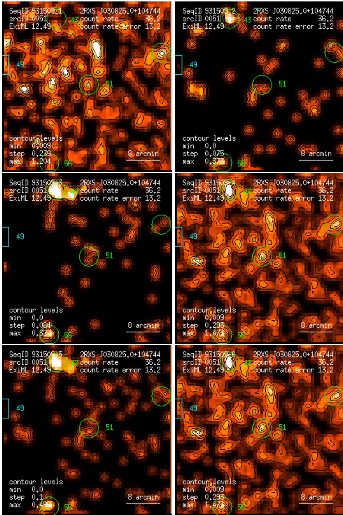
Figure 51: RASS 931509: detection 0051: band rate images, Gaussian filter: (1) PSPC channels 11 – 41, (2) 52 – 90, (3) 91 – 201, (4) 11 – 235, (5) 52 – 201, (6) 11 – 201. Broad band rates in counts/ks. Band rate contour levels in counts/ks/arcmin 2 .
