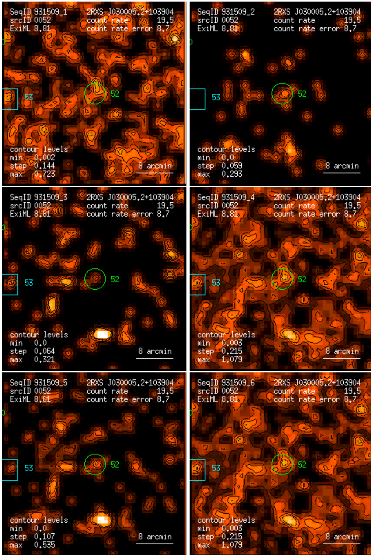
Figure 52: RASS 931509: detection 0052: band rate images, Gaussian filter: (1) PSPC channels 11 – 41, (2) 52 – 90, (3) 91 – 201, (4) 11 – 235, (5) 52 – 201, (6) 11 – 201. Broad band rates in counts/ks. Band rate contour levels in counts/ks/arcmin 2 .
