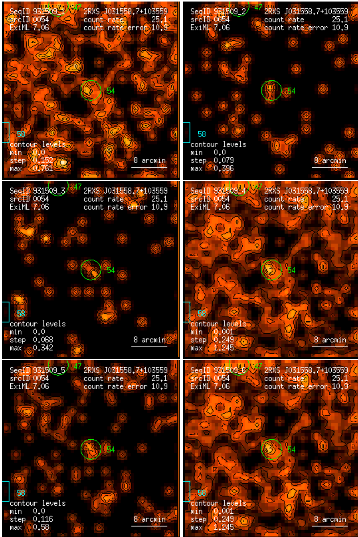
Figure 54: RASS 931509: detection 0054: band rate images, Gaussian filter: (1) PSPC channels 11 – 41, (2) 52 – 90, (3) 91 – 201, (4) 11 – 235, (5) 52 – 201, (6) 11 – 201. Broad band rates in counts/ks. Band rate contour levels in counts/ks/arcmin 2 .
