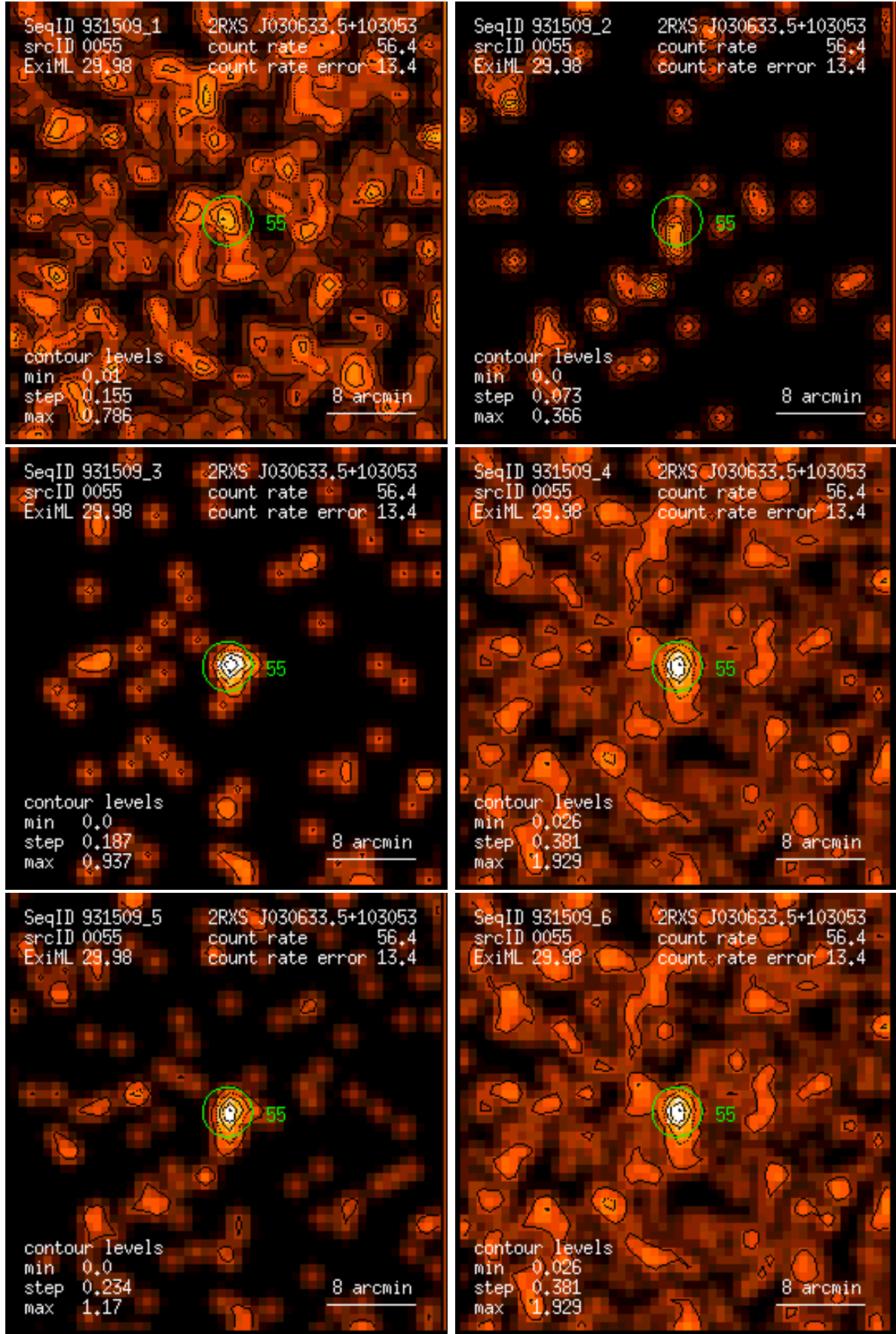
Figure 55: RASS 931509: detection 0055: band rate images, Gaussian filter: (1) PSPC channels 11 – 41, (2) 52 – 90, (3) 91 – 201, (4) 11 – 235, (5) 52 – 201, (6) 11 – 201. Broad band rates in counts/ks. Band rate contour levels in counts/ks/arcmin 2 .
