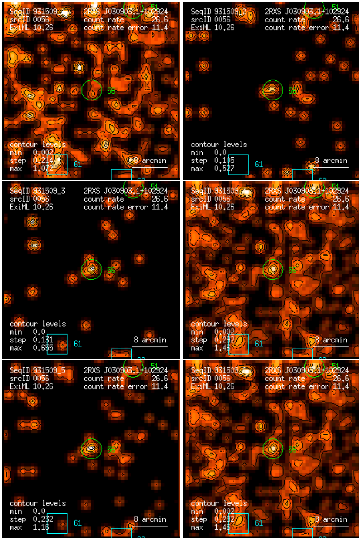
Figure 56: RASS 931509: detection 0056: band rate images, Gaussian filter: (1) PSPC channels 11 – 41, (2) 52 – 90, (3) 91 – 201, (4) 11 – 235, (5) 52 – 201, (6) 11 – 201. Broad band rates in counts/ks. Band rate contour levels in counts/ks/arcmin 2 .
