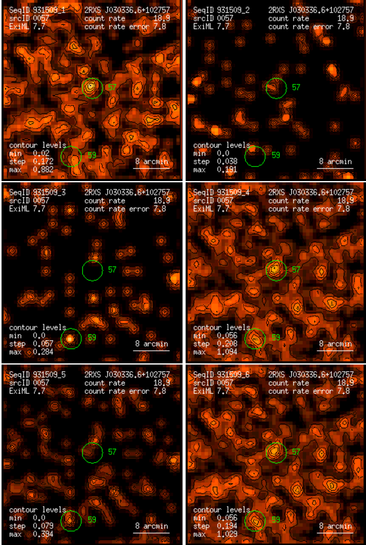
Figure 57: RASS 931509: detection 0057: band rate images, Gaussian filter: (1) PSPC channels 11 – 41, (2) 52 – 90, (3) 91 – 201, (4) 11 – 235, (5) 52 – 201, (6) 11 – 201. Broad band rates in counts/ks. Band rate contour levels in counts/ks/arcmin 2 .
