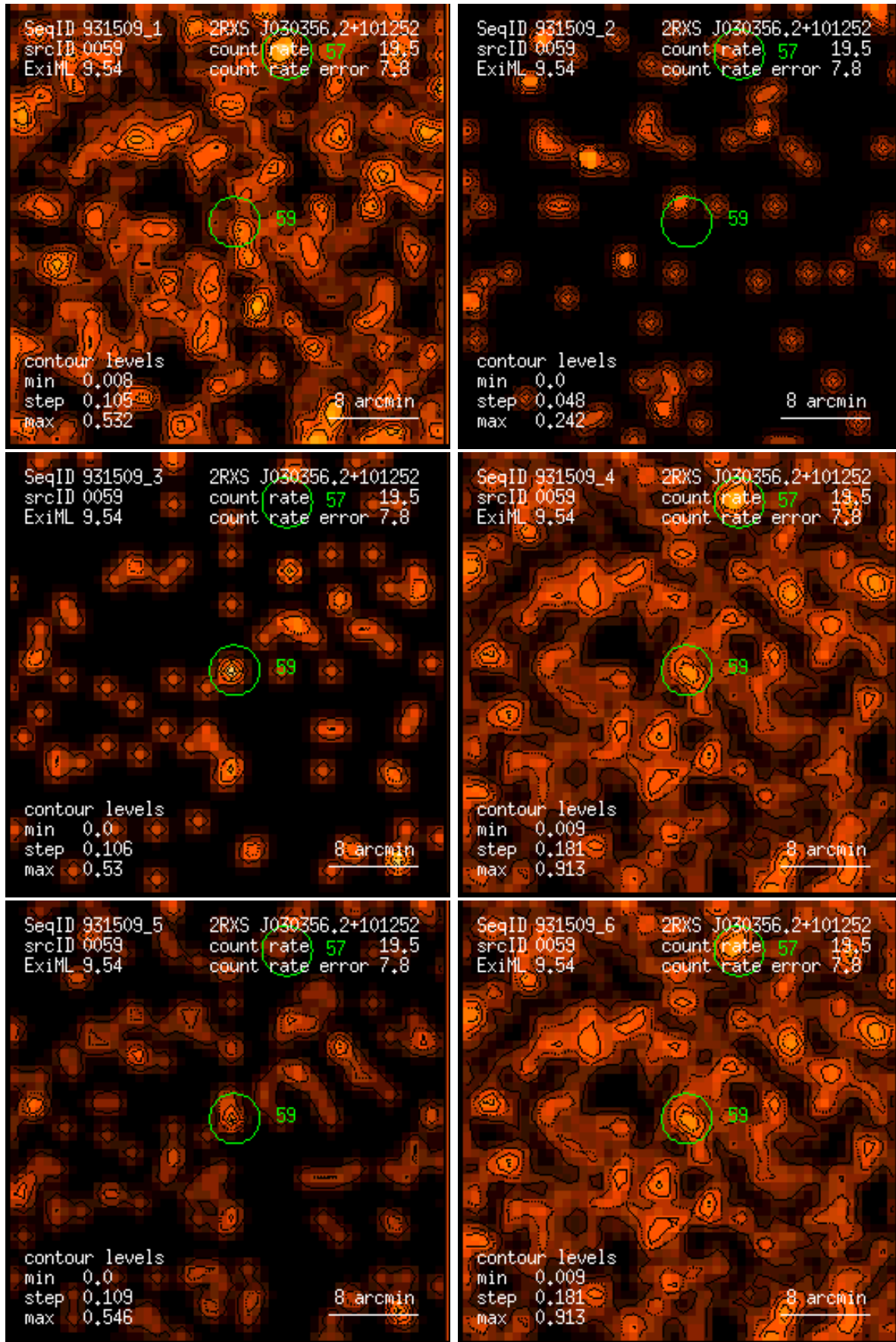
Figure 59: RASS 931509: detection 0059: band rate images, Gaussian filter: (1) PSPC channels 11 – 41, (2) 52 – 90, (3) 91 – 201, (4) 11 – 235, (5) 52 – 201, (6) 11 – 201. Broad band rates in counts/ks. Band rate contour levels in counts/ks/arcmin 2 .
