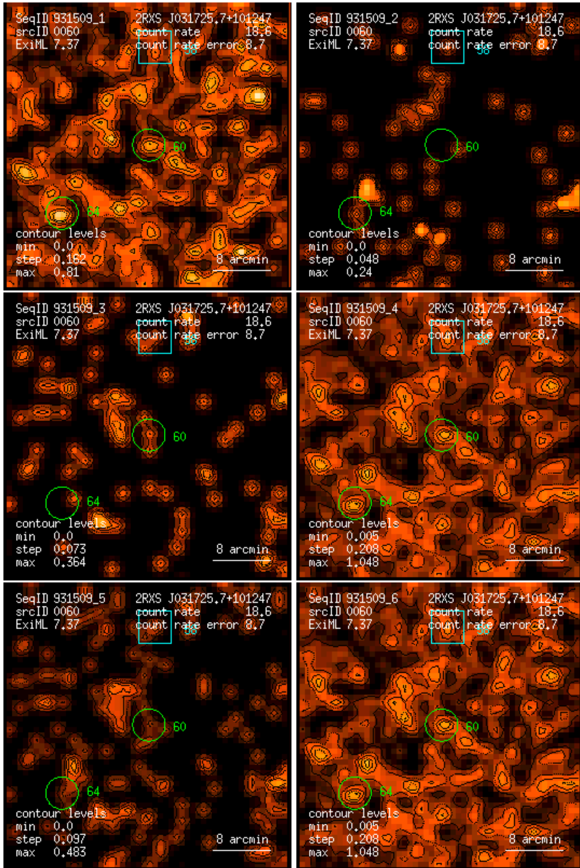
Figure 60: RASS 931509: detection 0060: band rate images, Gaussian filter: (1) PSPC channels 11 – 41, (2) 52 – 90, (3) 91 – 201, (4) 11 – 235, (5) 52 – 201, (6) 11 – 201. Broad band rates in counts/ks. Band rate contour levels in counts/ks/arcmin 2 .
