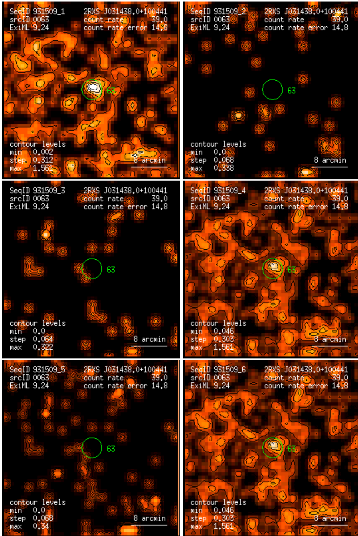
Figure 63: RASS 931509: detection 0063: band rate images, Gaussian filter: (1) PSPC channels 11 – 41, (2) 52 – 90, (3) 91 – 201, (4) 11 – 235, (5) 52 – 201, (6) 11 – 201. Broad band rates in counts/ks. Band rate contour levels in counts/ks/arcmin 2 .
