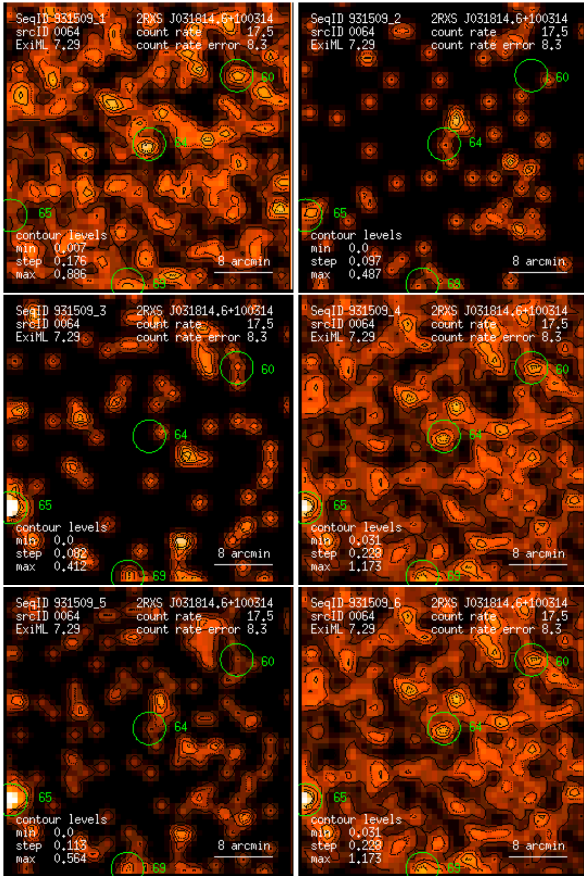
Figure 64: RASS 931509: detection 0064: band rate images, Gaussian filter: (1) PSPC channels 11 – 41, (2) 52 – 90, (3) 91 – 201, (4) 11 – 235, (5) 52 – 201, (6) 11 – 201. Broad band rates in counts/ks. Band rate contour levels in counts/ks/arcmin 2 .
