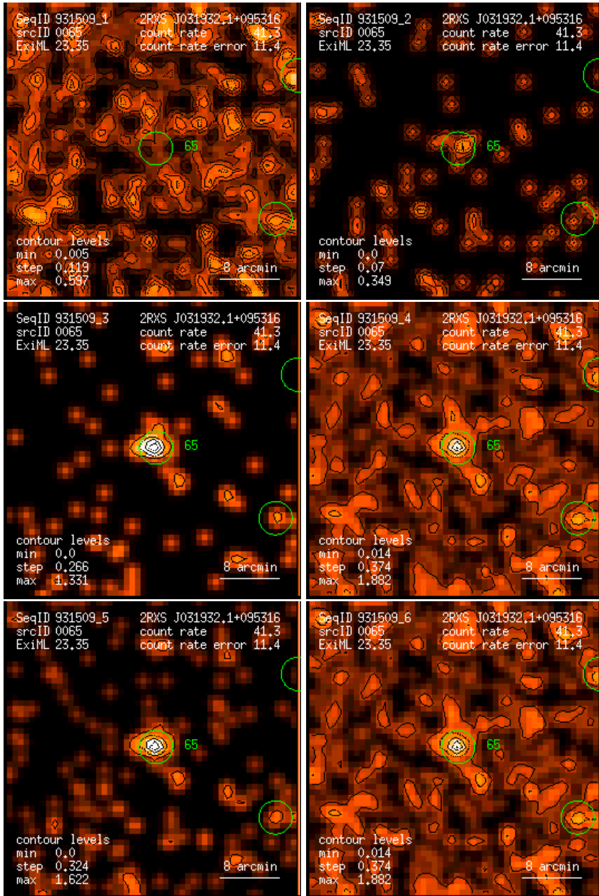
Figure 65: RASS 931509: detection 0065: band rate images, Gaussian filter: (1) PSPC channels 11 – 41, (2) 52 – 90, (3) 91 – 201, (4) 11 – 235, (5) 52 – 201, (6) 11 – 201. Broad band rates in counts/ks. Band rate contour levels in counts/ks/arcmin 2 .
