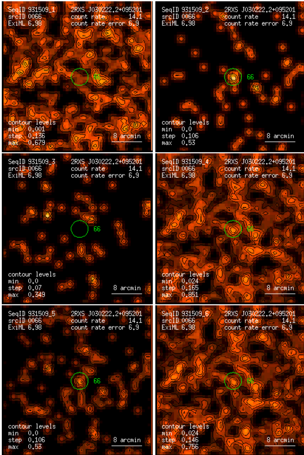
Figure 66: RASS 931509: detection 0066: band rate images, Gaussian filter: (1) PSPC channels 11 – 41, (2) 52 – 90, (3) 91 – 201, (4) 11 – 235, (5) 52 – 201, (6) 11 – 201. Broad band rates in counts/ks. Band rate contour levels in counts/ks/arcmin 2 .
