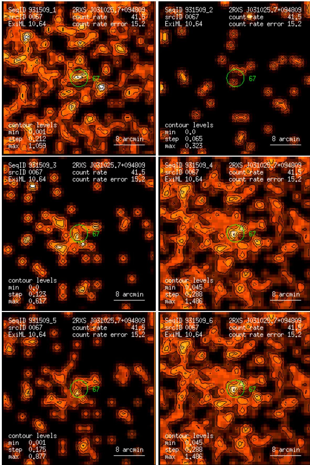
Figure 67: RASS 931509: detection 0067: band rate images, Gaussian filter: (1) PSPC channels 11 – 41, (2) 52 – 90, (3) 91 – 201, (4) 11 – 235, (5) 52 – 201, (6) 11 – 201. Broad band rates in counts/ks. Band rate contour levels in counts/ks/arcmin 2 .
