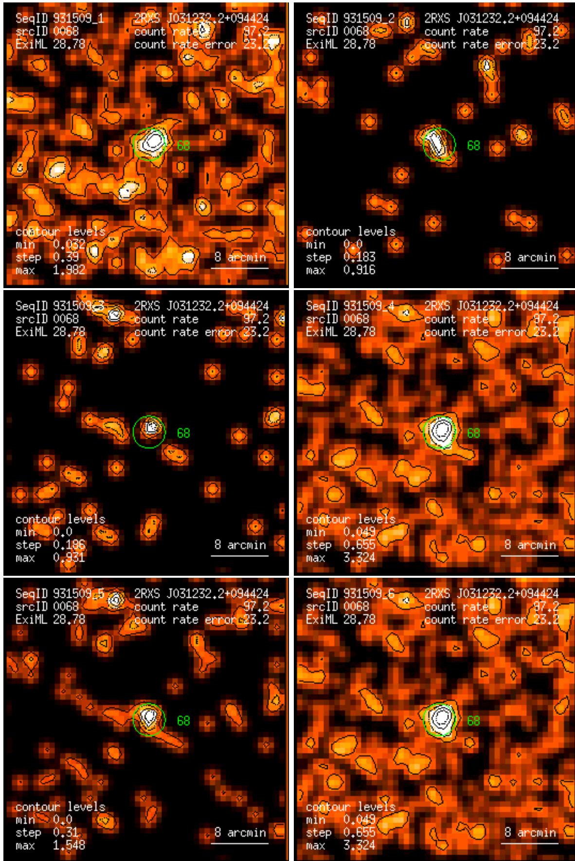
Figure 68: RASS 931509: detection 0068: band rate images, Gaussian filter: (1) PSPC channels 11 – 41, (2) 52 – 90, (3) 91 – 201, (4) 11 – 235, (5) 52 – 201, (6) 11 – 201. Broad band rates in counts/ks. Band rate contour levels in counts/ks/arcmin 2 .
