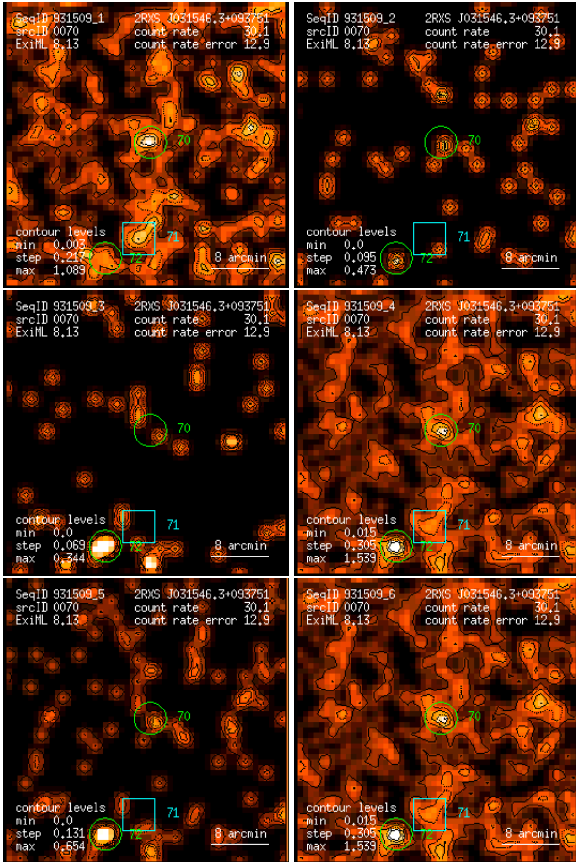
Figure 70: RASS 931509: detection 0070: band rate images, Gaussian filter: (1) PSPC channels 11 – 41, (2) 52 – 90, (3) 91 – 201, (4) 11 – 235, (5) 52 – 201, (6) 11 – 201. Broad band rates in counts/ks. Band rate contour levels in counts/ks/arcmin 2 .
