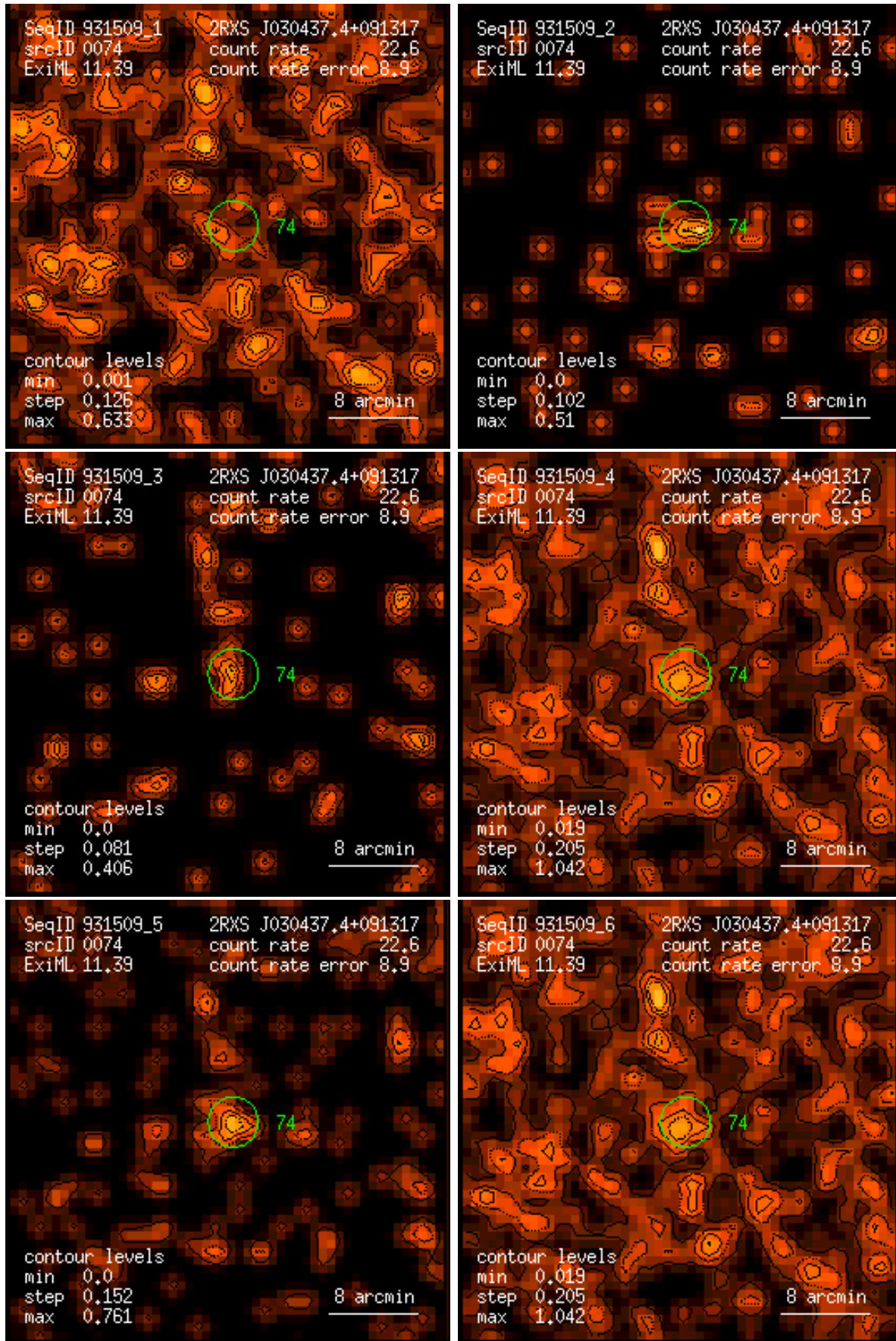
Figure 74: RASS 931509: detection 0074: band rate images, Gaussian filter: (1) PSPC channels 11 – 41, (2) 52 – 90, (3) 91 – 201, (4) 11 – 235, (5) 52 – 201, (6) 11 – 201. Broad band rates in counts/ks. Band rate contour levels in counts/ks/arcmin 2 .
