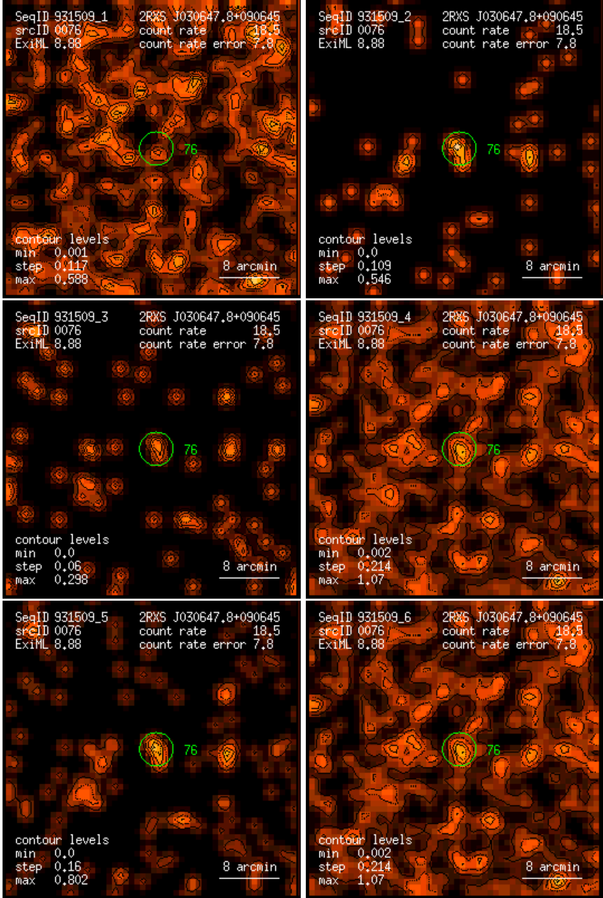
Figure 76: RASS 931509: detection 0076: band rate images, Gaussian filter: (1) PSPC channels 11 – 41, (2) 52 – 90, (3) 91 – 201, (4) 11 – 235, (5) 52 – 201, (6) 11 – 201. Broad band rates in counts/ks. Band rate contour levels in counts/ks/arcmin 2 .
