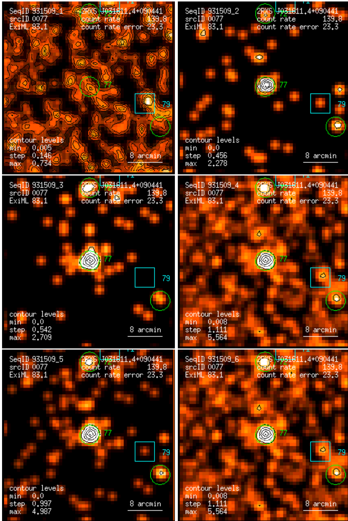
Figure 77: RASS 931509: detection 0077: band rate images, Gaussian filter: (1) PSPC channels 11 – 41, (2) 52 – 90, (3) 91 – 201, (4) 11 – 235, (5) 52 – 201, (6) 11 – 201. Broad band rates in counts/ks. Band rate contour levels in counts/ks/arcmin 2 .
