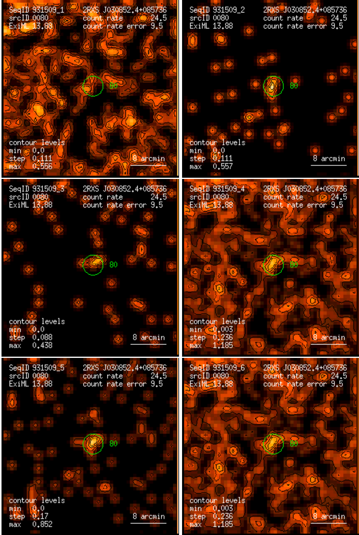
Figure 80: RASS 931509: detection 0080: band rate images, Gaussian filter: (1) PSPC channels 11 – 41, (2) 52 – 90, (3) 91 – 201, (4) 11 – 235, (5) 52 – 201, (6) 11 – 201. Broad band rates in counts/ks. Band rate contour levels in counts/ks/arcmin 2 .
