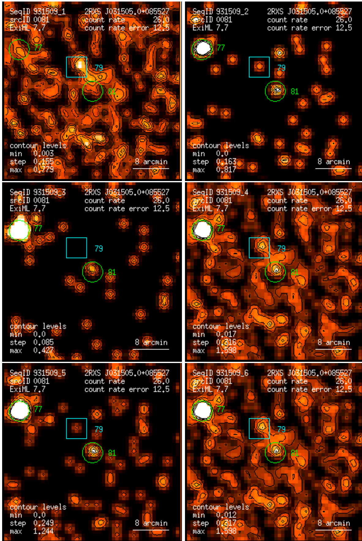
Figure 81: RASS 931509: detection 0081: band rate images, Gaussian filter: (1) PSPC channels 11 – 41, (2) 52 – 90, (3) 91 – 201, (4) 11 – 235, (5) 52 – 201, (6) 11 – 201. Broad band rates in counts/ks. Band rate contour levels in counts/ks/arcmin 2 .
