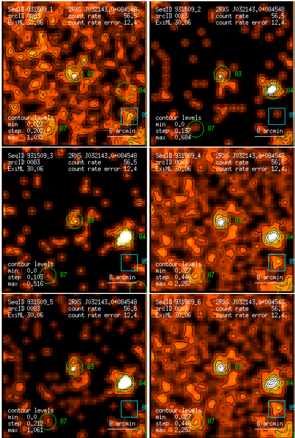
Figure 83: RASS 931509: detection 0083: band rate images, Gaussian filter: (1) PSPC channels 11 – 41, (2) 52 – 90, (3) 91 – 201, (4) 11 – 235, (5) 52 – 201, (6) 11 – 201. Broad band rates in counts/ks. Band rate contour levels in counts/ks/arcmin 2 .
