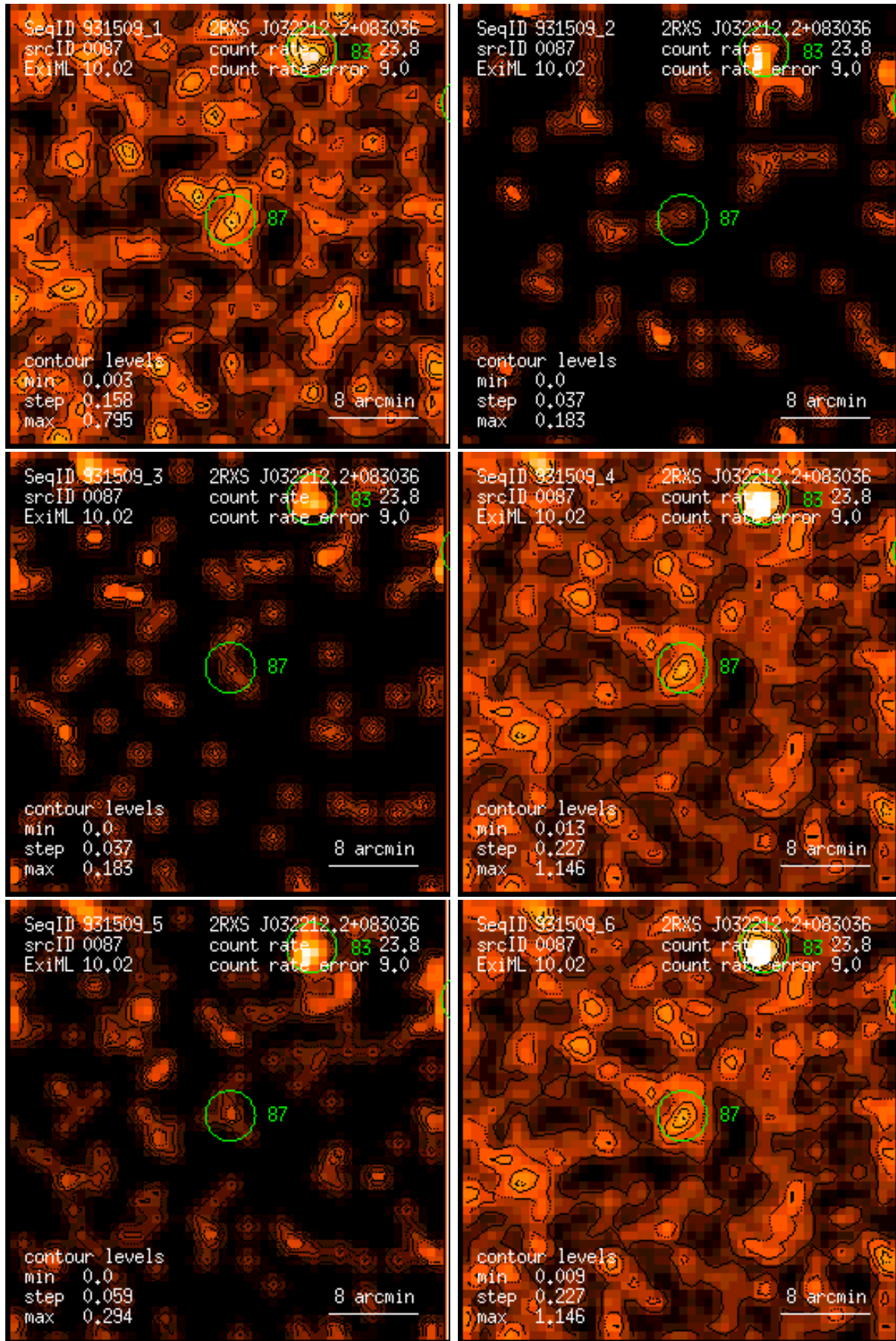
Figure 87: RASS 931509: detection 0087: band rate images, Gaussian filter: (1) PSPC channels 11 – 41, (2) 52 – 90, (3) 91 – 201, (4) 11 – 235, (5) 52 – 201, (6) 11 – 201. Broad band rates in counts/ks. Band rate contour levels in counts/ks/arcmin 2 .
