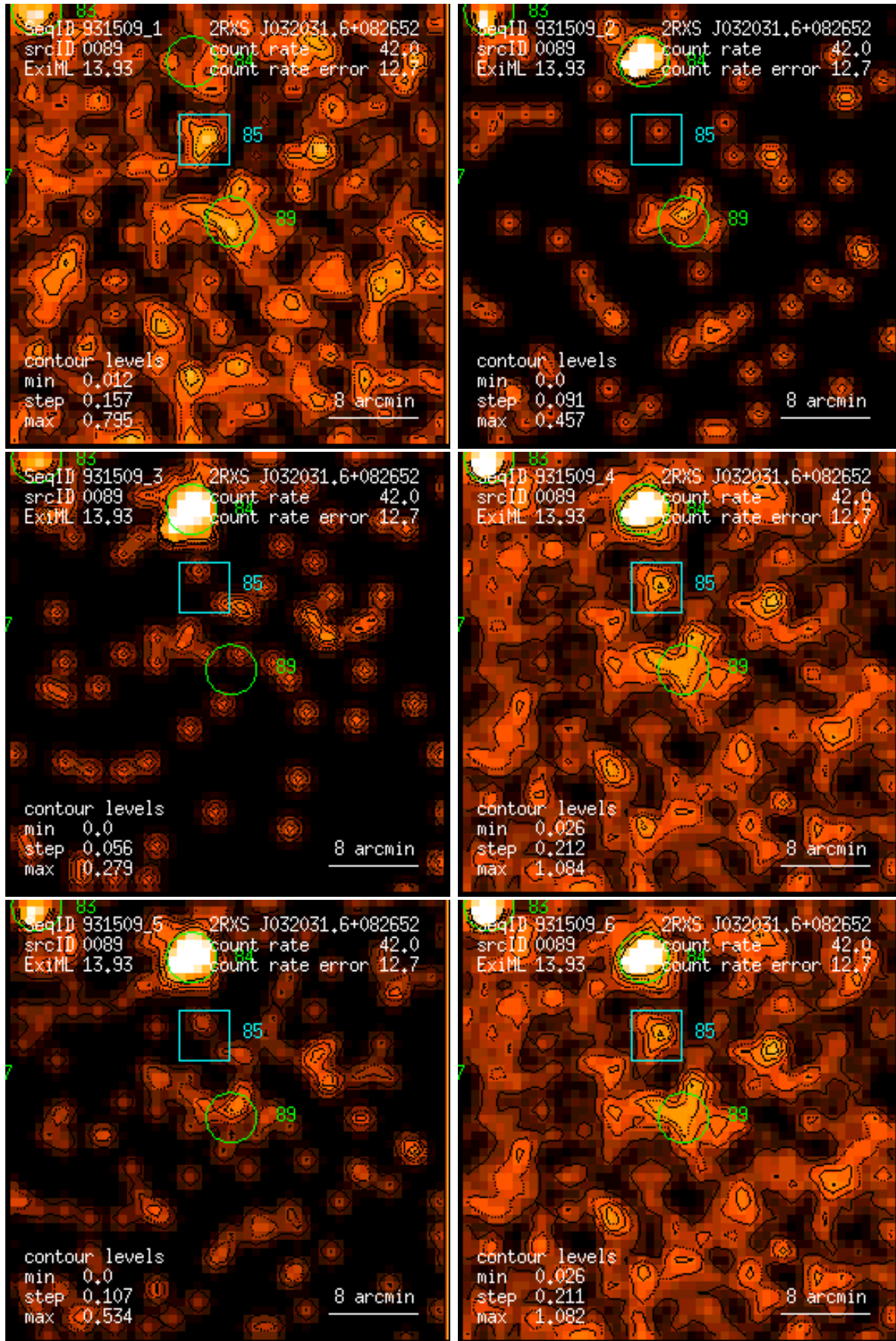
Figure 89: RASS 931509: detection 0089: band rate images, Gaussian filter: (1) PSPC channels 11 – 41, (2) 52 – 90, (3) 91 – 201, (4) 11 – 235, (5) 52 – 201, (6) 11 – 201. Broad band rates in counts/ks. Band rate contour levels in counts/ks/arcmin 2 .
