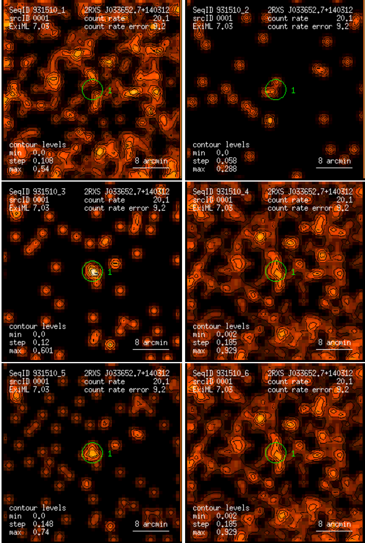
Figure 1: RASS 931510: detection 0001: band rate images, Gaussian filter: (1) PSPC channels 11 – 41, (2) 52 – 90, (3) 91 – 201, (4) 11 – 235, (5) 52 – 201, (6) 11 – 201. Broad band rates in counts/ks. Band rate contour levels in counts/ks/arcmin 2 .
