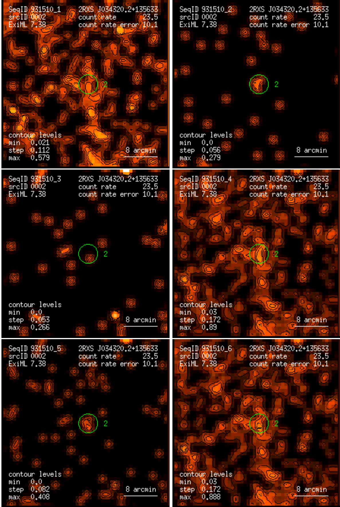
Figure 2: RASS 931510: detection 0002: band rate images, Gaussian filter: (1) PSPC channels 11 – 41, (2) 52 – 90, (3) 91 – 201, (4) 11 – 235, (5) 52 – 201, (6) 11 – 201. Broad band rates in counts/ks. Band rate contour levels in counts/ks/arcmin 2 .
