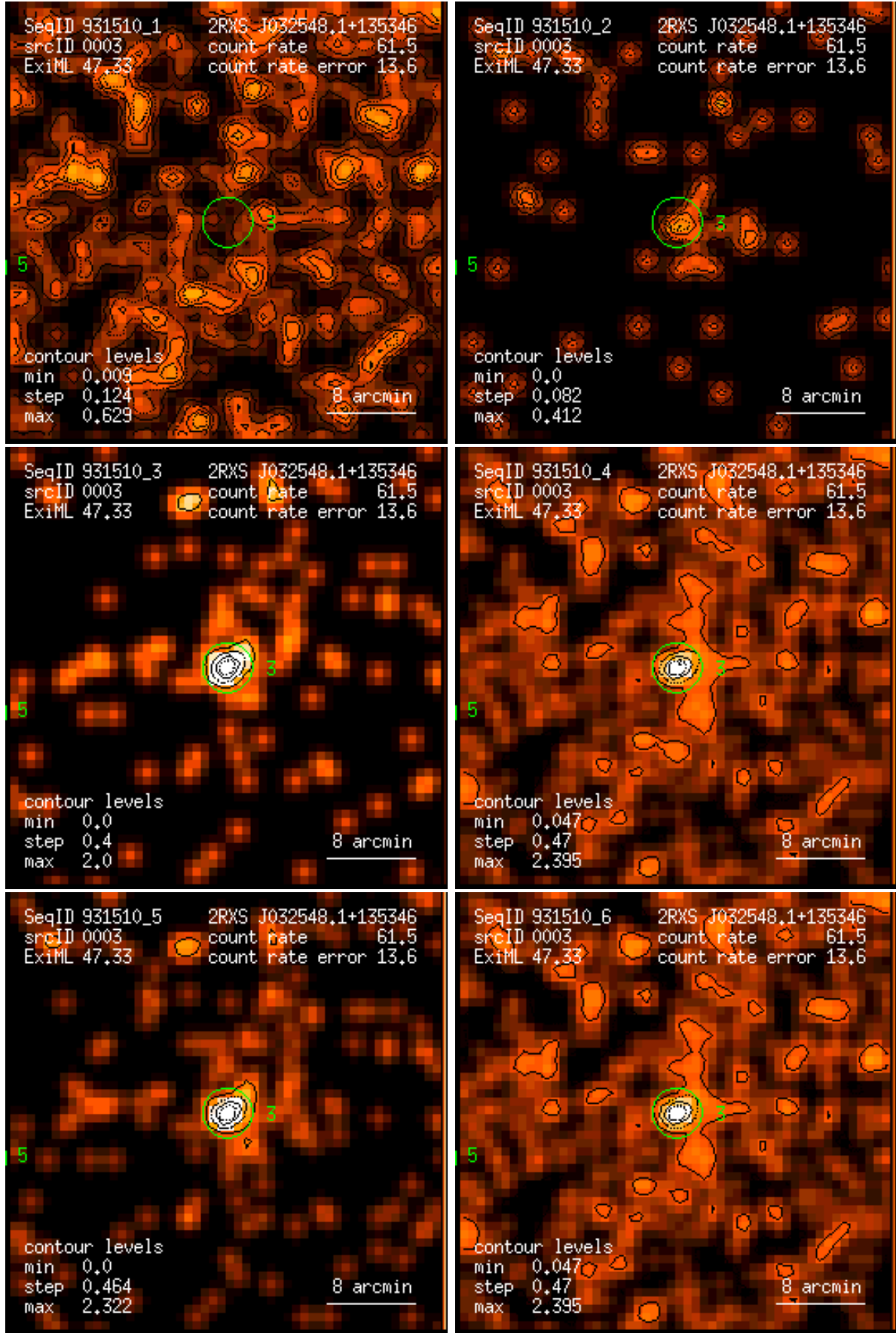
Figure 3: RASS 931510: detection 0003: band rate images, Gaussian filter: (1) PSPC channels 11 – 41, (2) 52 – 90, (3) 91 – 201, (4) 11 – 235, (5) 52 – 201, (6) 11 – 201. Broad band rates in counts/ks. Band rate contour levels in counts/ks/arcmin 2 .
