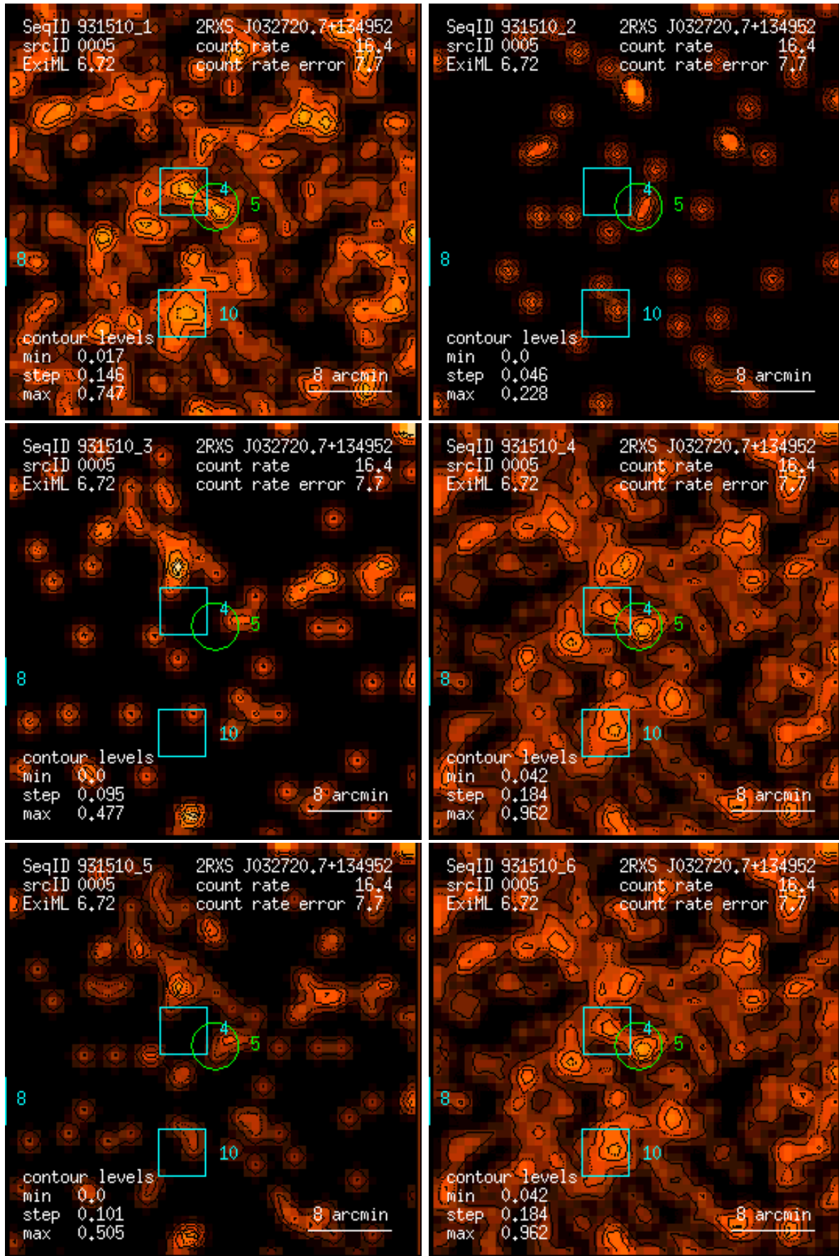
Figure 5: RASS 931510: detection 0005: band rate images, Gaussian filter: (1) PSPC channels 11 – 41, (2) 52 – 90, (3) 91 – 201, (4) 11 – 235, (5) 52 – 201, (6) 11 – 201. Broad band rates in counts/ks. Band rate contour levels in counts/ks/arcmin 2 .
