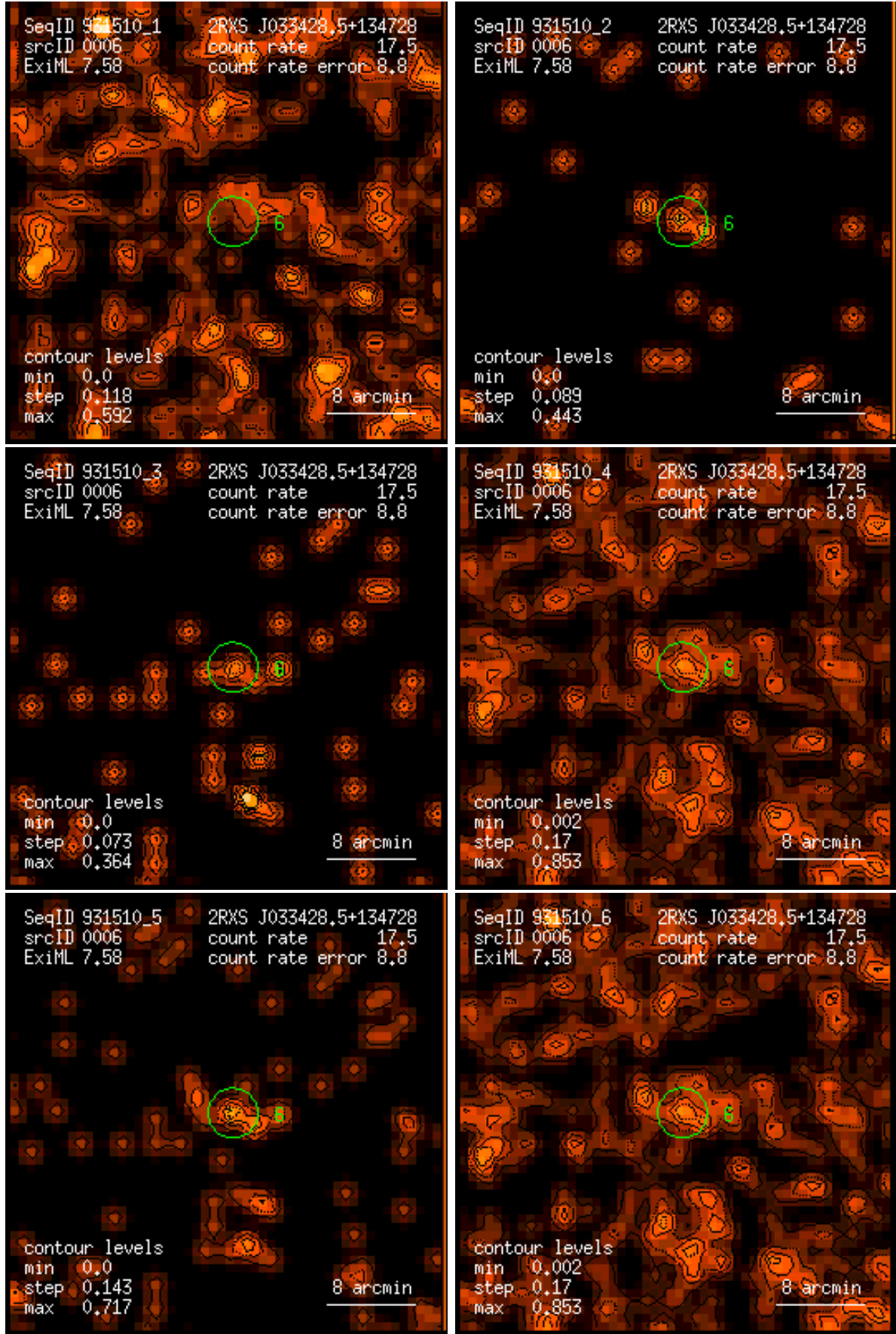
Figure 6: RASS 931510: detection 0006: band rate images, Gaussian filter: (1) PSPC channels 11 – 41, (2) 52 – 90, (3) 91 – 201, (4) 11 – 235, (5) 52 – 201, (6) 11 – 201. Broad band rates in counts/ks. Band rate contour levels in counts/ks/arcmin 2 .
