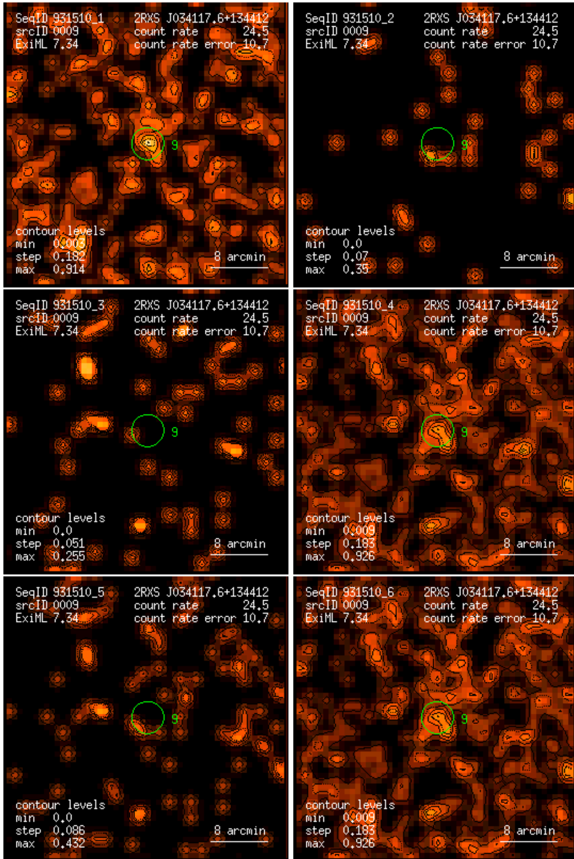
Figure 9: RASS 931510: detection 0009: band rate images, Gaussian filter: (1) PSPC channels 11 – 41, (2) 52 – 90, (3) 91 – 201, (4) 11 – 235, (5) 52 – 201, (6) 11 – 201. Broad band rates in counts/ks. Band rate contour levels in counts/ks/arcmin 2 .
