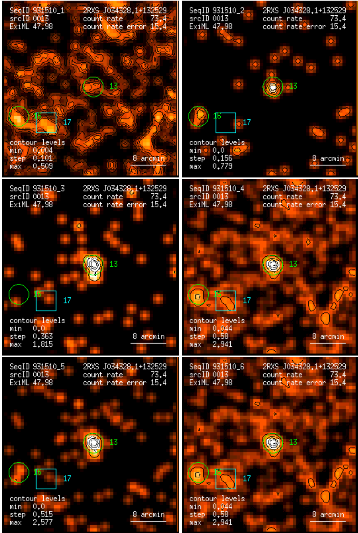
Figure 13: RASS 931510: detection 0013: band rate images, Gaussian filter: (1) PSPC channels 11 – 41, (2) 52 – 90, (3) 91 – 201, (4) 11 – 235, (5) 52 – 201, (6) 11 – 201. Broad band rates in counts/ks. Band rate contour levels in counts/ks/arcmin 2 .
